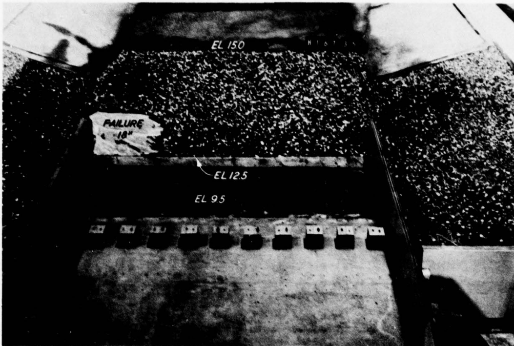
Figure 9. Failure of 18-in. riprap after 30-min (prototype) operation with design flow 28,900 cfs
