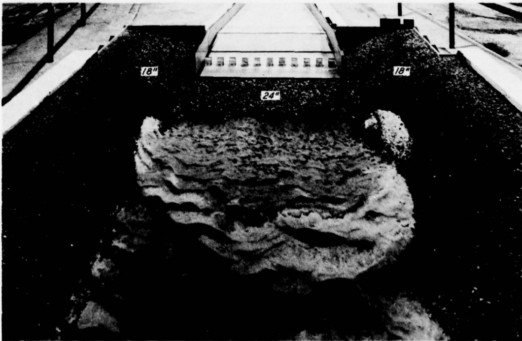
Photo 21. Stilling basin B-1 (type 5) after 1-hr (prototype) operation; type 7 riprap plan, 18-in. riprap on slopes, 24-in. riprap on bottom (el 11.5)
