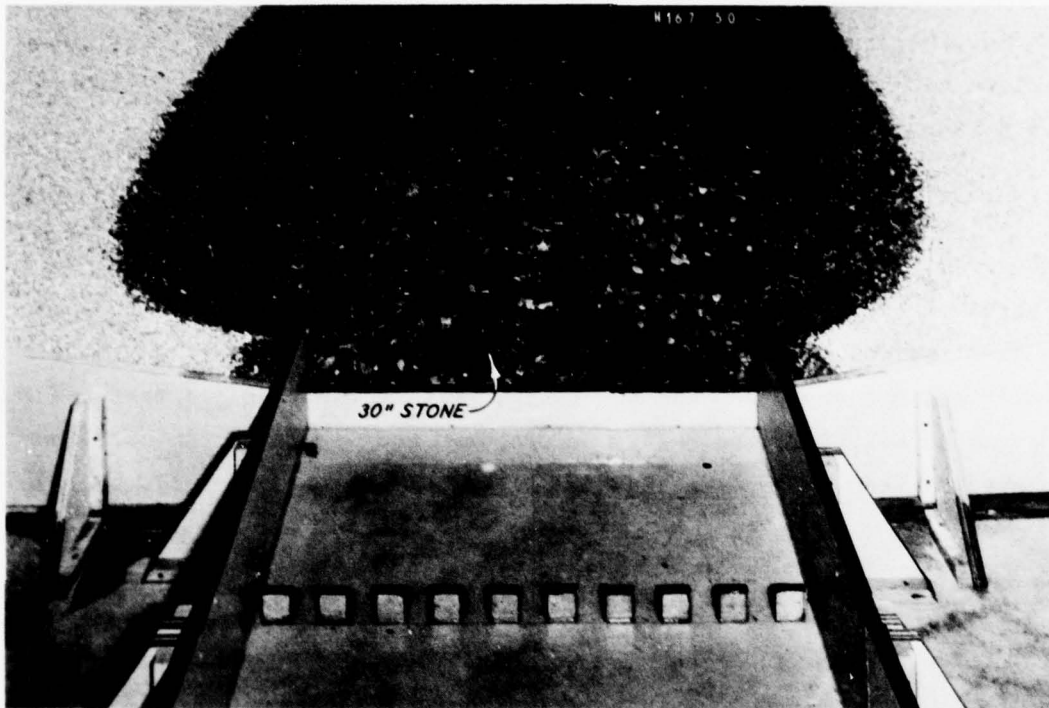
Figure 8. Dry bed of original stilling basin B-3 showing riprap damage after 1-hr (prototype) operation with design flow 22,700 cfs and tailwater el 129.5
