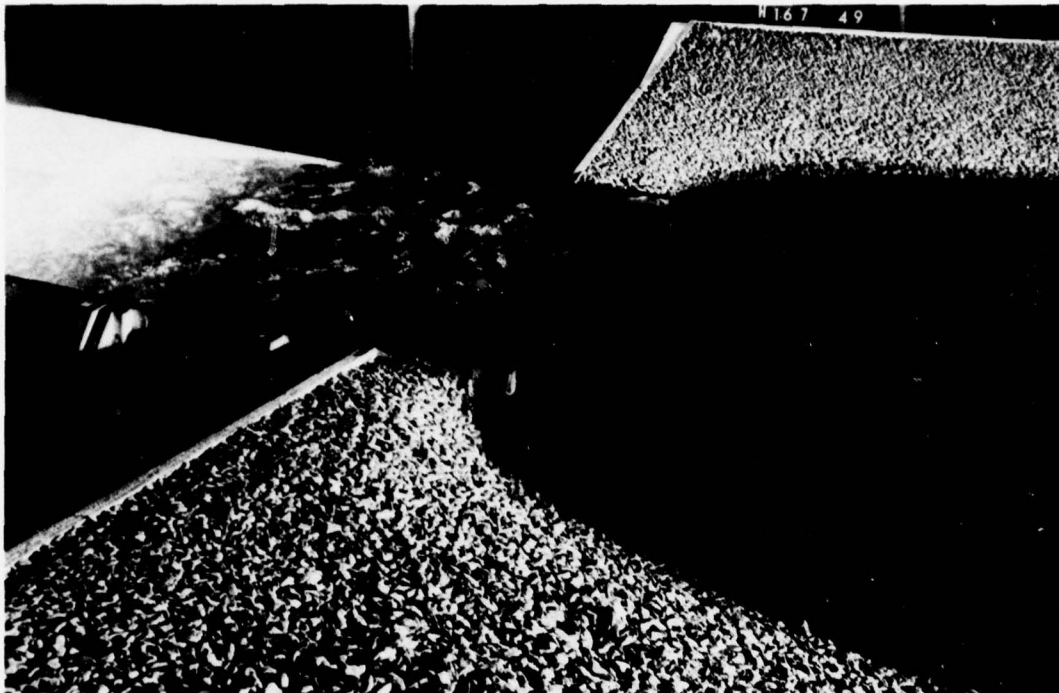
Photo 20. Stilling basin B-3 (original design); design flow 22,700 cfs, tailwater el 129.5
