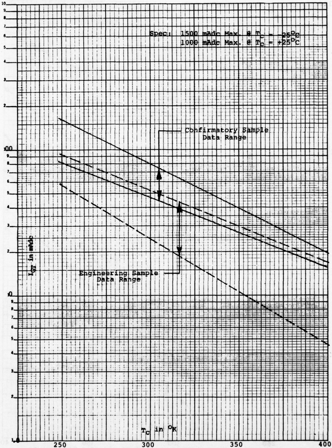
Fig. 7 Gate Trigger Current vs. Case Temperature 36
