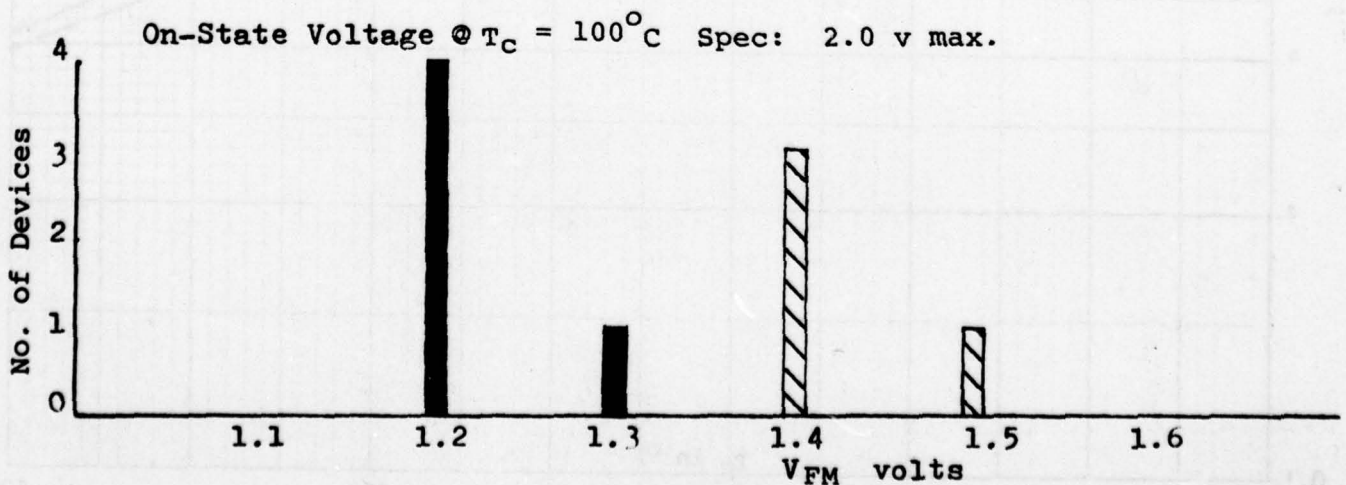
Fig. 9 Confirmatory/Engineering Tests
