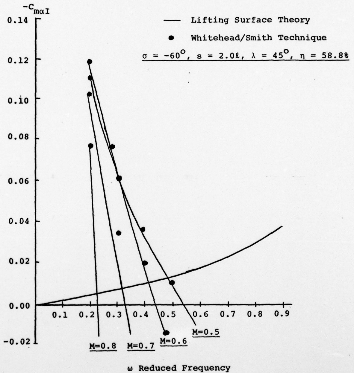
Figure 1. Torsional Flutter Boundaries
