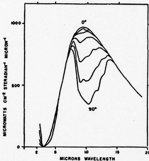
Fig. 5. The spectral radiance of the sky covered with cirrus clouds at several elevations. (Ref 7:1318)
