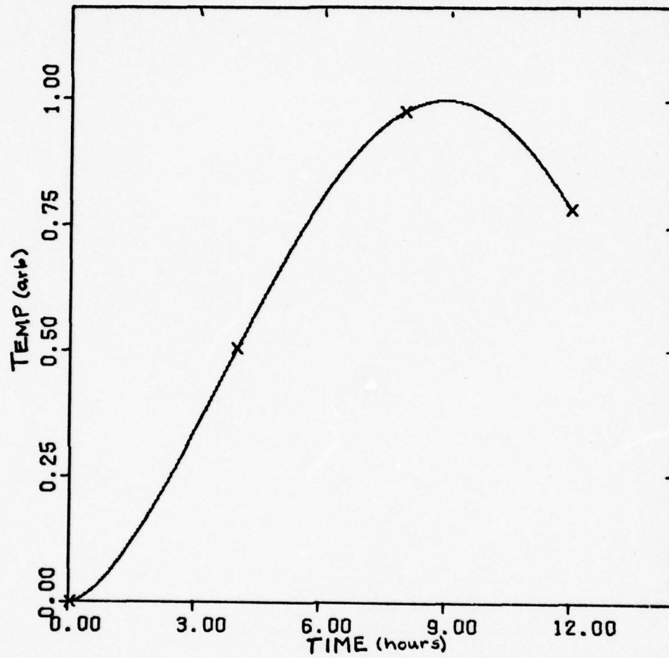
Fig. 22 Eq. (14) solution to semi-infinite slab problem, with DT=0.02 .
