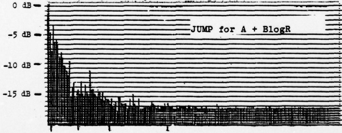
Figure 4-7 Spectra of TL Fluctuations (see Figures 4-5 and 4-6) (Over 100-500 nm Interval)
