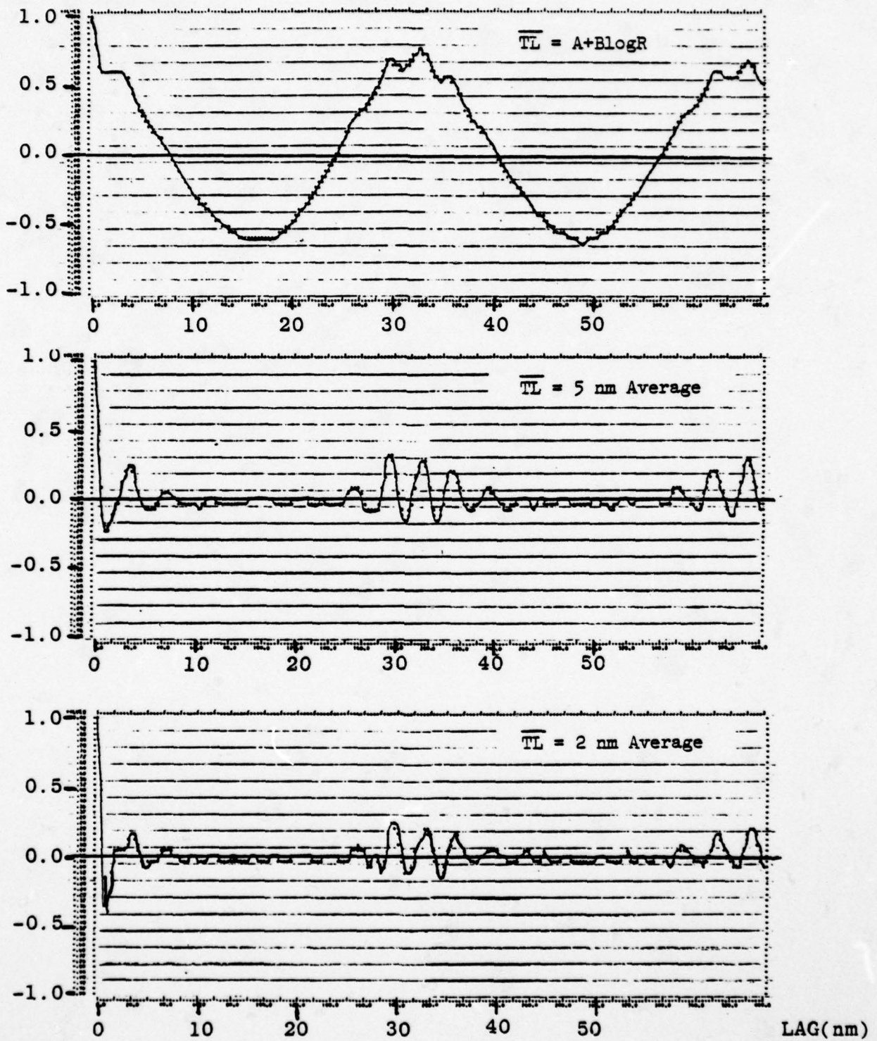
Autocovariance Functions for TL Fluctuations Over Range Interval 100-500 nm
