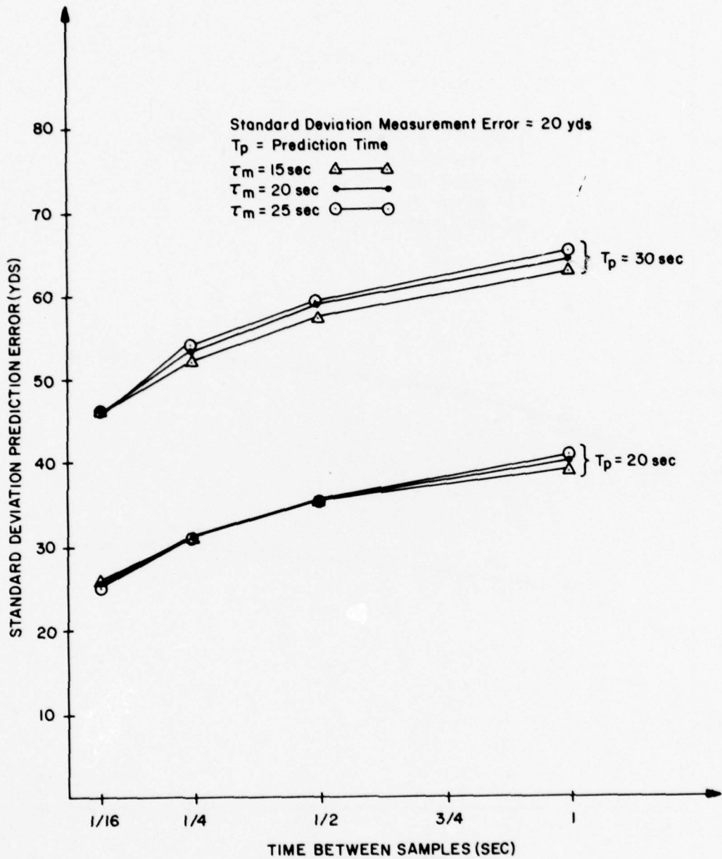
Figure 6. Prediction Error Covariance Sensitivity with Respect to \tau_m (surface target)
