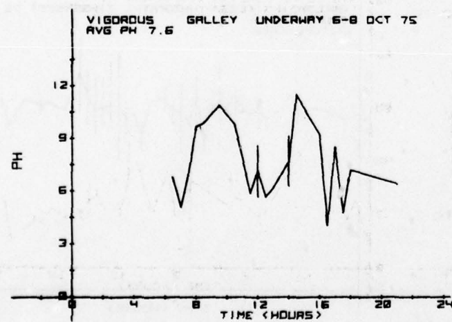
FIGURE 70. UNDERWAY GALLEY pH
