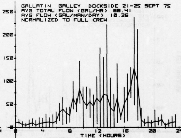
FIGURE 49. NORMALIZED GALLEY WASTEWATER FLOW; SEGMENTED, DOCKSIDE
