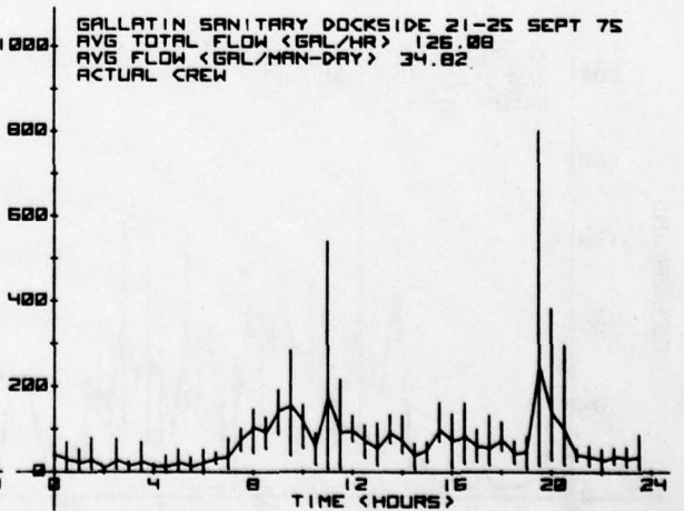
FIGURE 29. ACTUAL SANITARY WASTEWATER FLOW; SEGMENTED, DOCKSIDE
