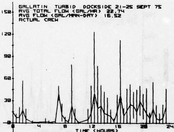
FIGURE 37. ACTUAL TURBID WASTEWATER FLOW; SEGMENTED, DOCKSIDE
