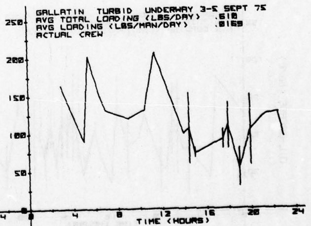
FIGURE 74. UNDERWAY TURBID OIL & GREASE LOADS
