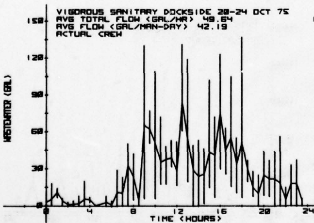
FIGURE 29. ACTUAL SANITARY WASTEWATER FLOW; SEGMENTED, DOCKSIDE
