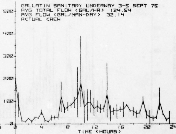
FIGURE 30. ACTUAL SANITARY WASTEWATER FLOW; SEGMENTED, UNDERWAY
