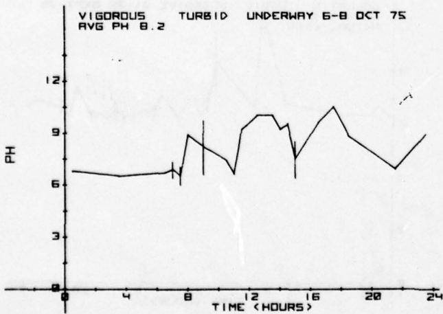
FIGURE 68. UNDERWAY TURBID pH 120
