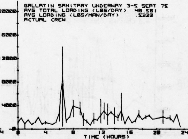
FIGURE 84. UNDERWAY SANITARY COD LOADS
