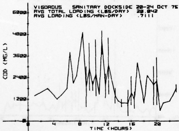
FIGURE 83. DOCKSIDE SANITARY COD LOADS
