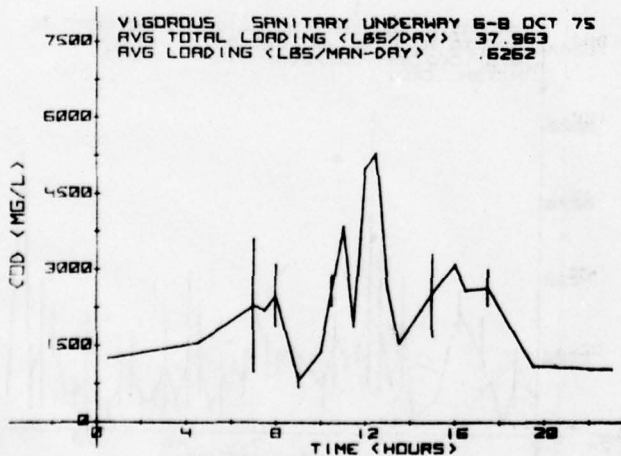
FIGURE 84. UNDERWAY SANITARY COD LOADS
