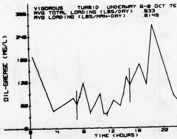
FIGURE 74. UNDERWAY TURBID OIL & GREASE LOADS
