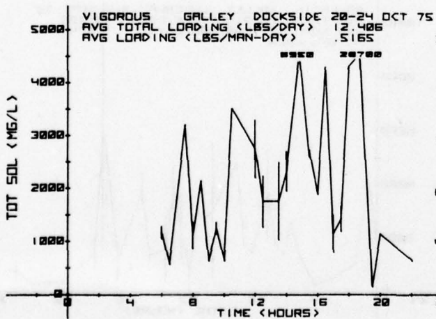
FIGURE 57. DOCKSIDE GALLEY TOTAL SOLIDS LOADS
