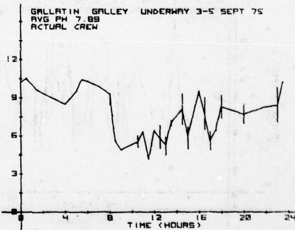
FIGURE 70. UNDERWAY GALLEY pH
