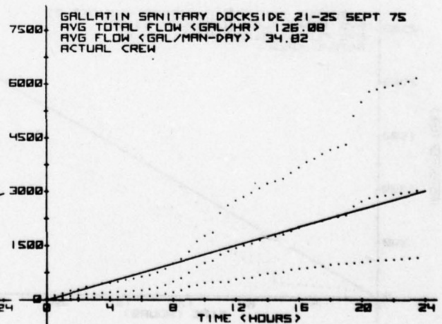
FIGURE 31. ACTUAL SANITARY WASTEWATER FLOW; CUMULATIVE, DOCKSIDE
