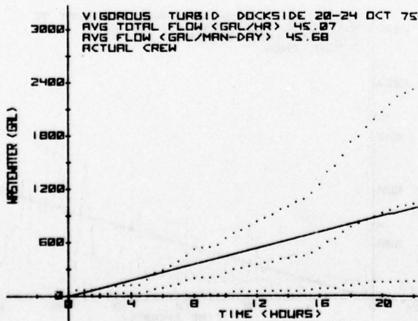
FIGURE 39. ACTUAL TURBID WASTEWATER FLOW; CUMULATIVE, DOCKSIDE
