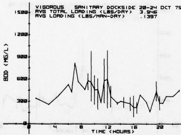
FIGURE 89. DOCKSIDE SANITARY BOD LOADS
