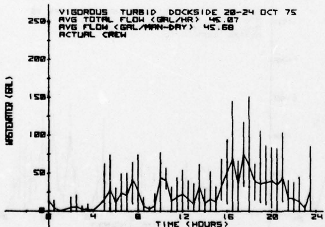
FIGURE 37. ACTUAL TURBID WASTEWATER FLOW; SEGMENTED, DOCKSIDE
