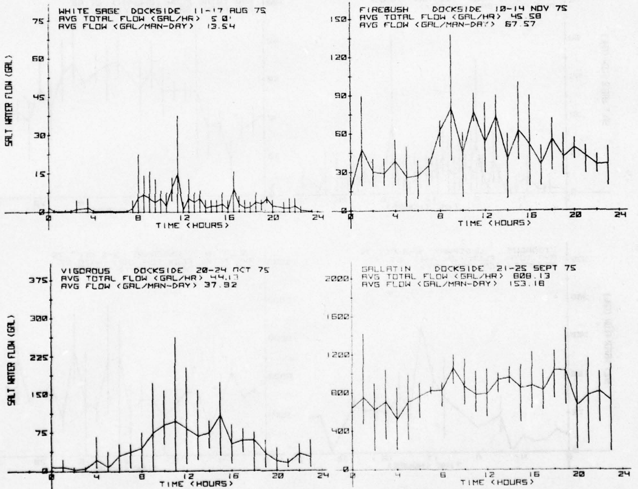
FIGURE 17. DOCKSIDE SEGMENTED SALT WATER USAGE
