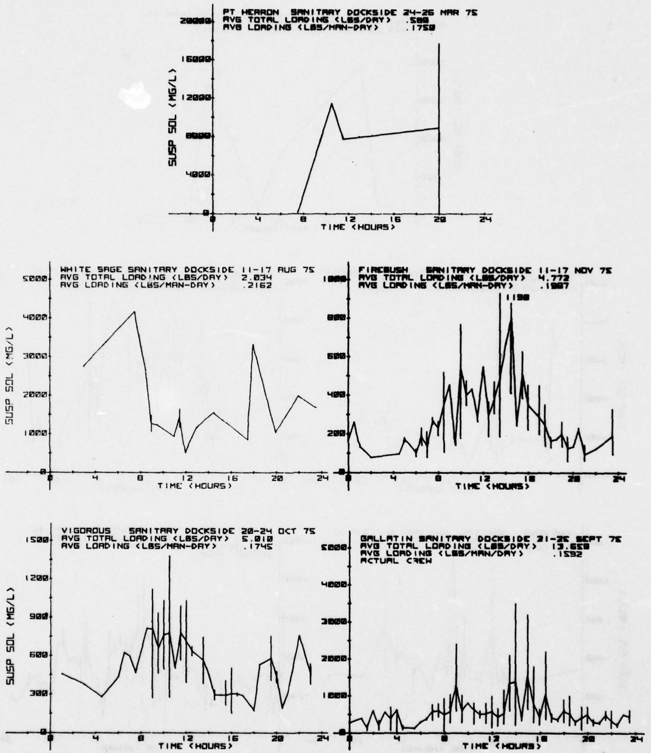
FIGURE 59. DOCKSIDE SANITARY SUSPENDED SOLIDS LOADS
