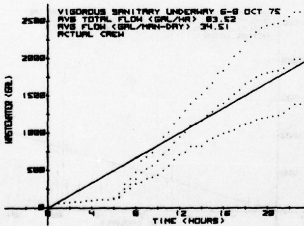
FIGURE 32. ACTUAL SANITARY WASTEWATER FLOW; CUMULATIVE, UNDERWAY
