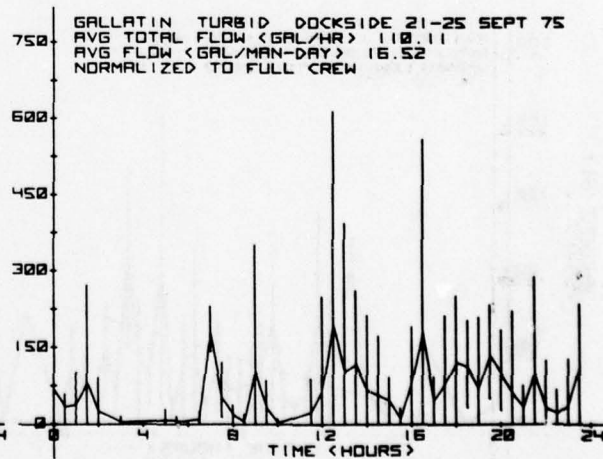
FIGURE 41. NORMALIZED TURBID WASTEWATER FLOW; SEGMENTED, DOCKSIDE
