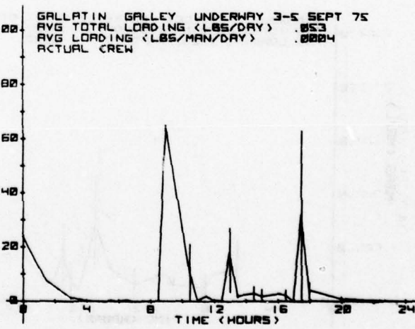
FIGURE 80. UNDERWAY GALLEY MBAS LOADS
