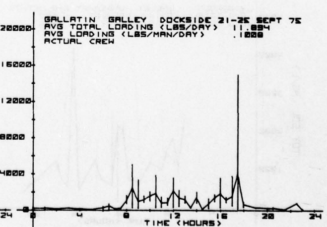
FIGURE 57. DOCKSIDE GALLEY TOTAL SOLIDS LOADS
