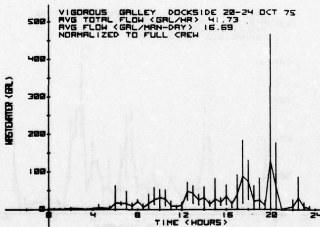
FIGURE 49. NORMALIZED GALLEY WASTEWATER FLOW; SEGMENTED, DOCKSIDE
