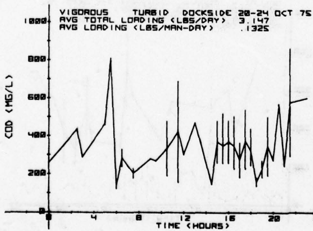
FIGURE 85. DOCKSIDE TURBID COD LOADS
