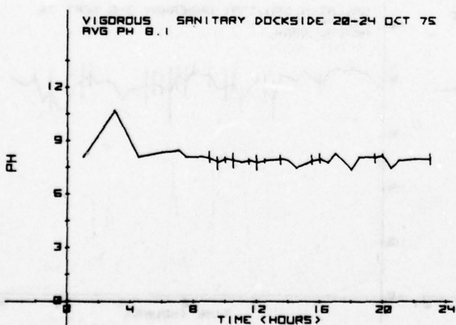
FIGURE 65. DOCKSIDE SANITARY pH
