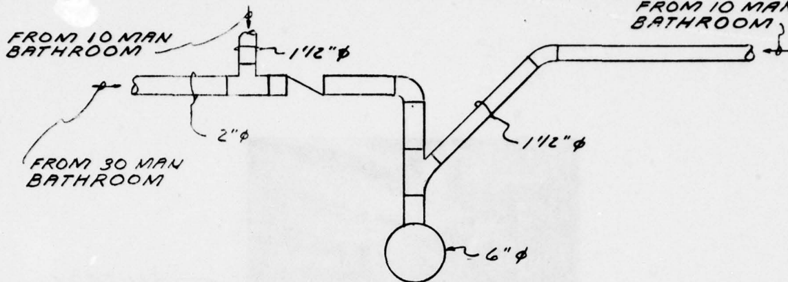
EXISTING TURBID WATER PIPING
