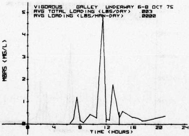
FIGURE 80. UNDERWAY GALLEY MBAS LOADS
