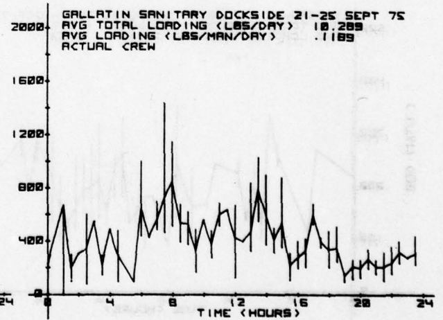
FIGURE 89. DOCKSIDE SANITARY BOD LOADS
