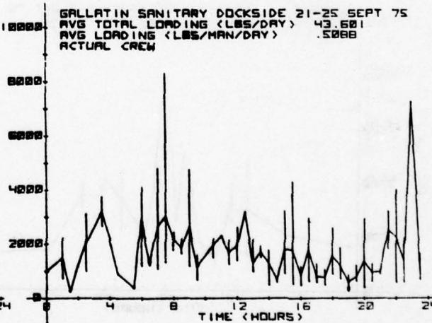
FIGURE 83. DOCKSIDE SANITARY COD LOADS
