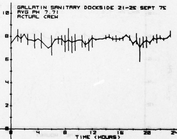
FIGURE 65. DOCKSIDE SANITARY pH
