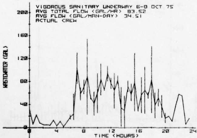
FIGURE 30. ACTUAL SANITARY WASTEWATER FLOW; SEGMENTED, UNDERWAY
