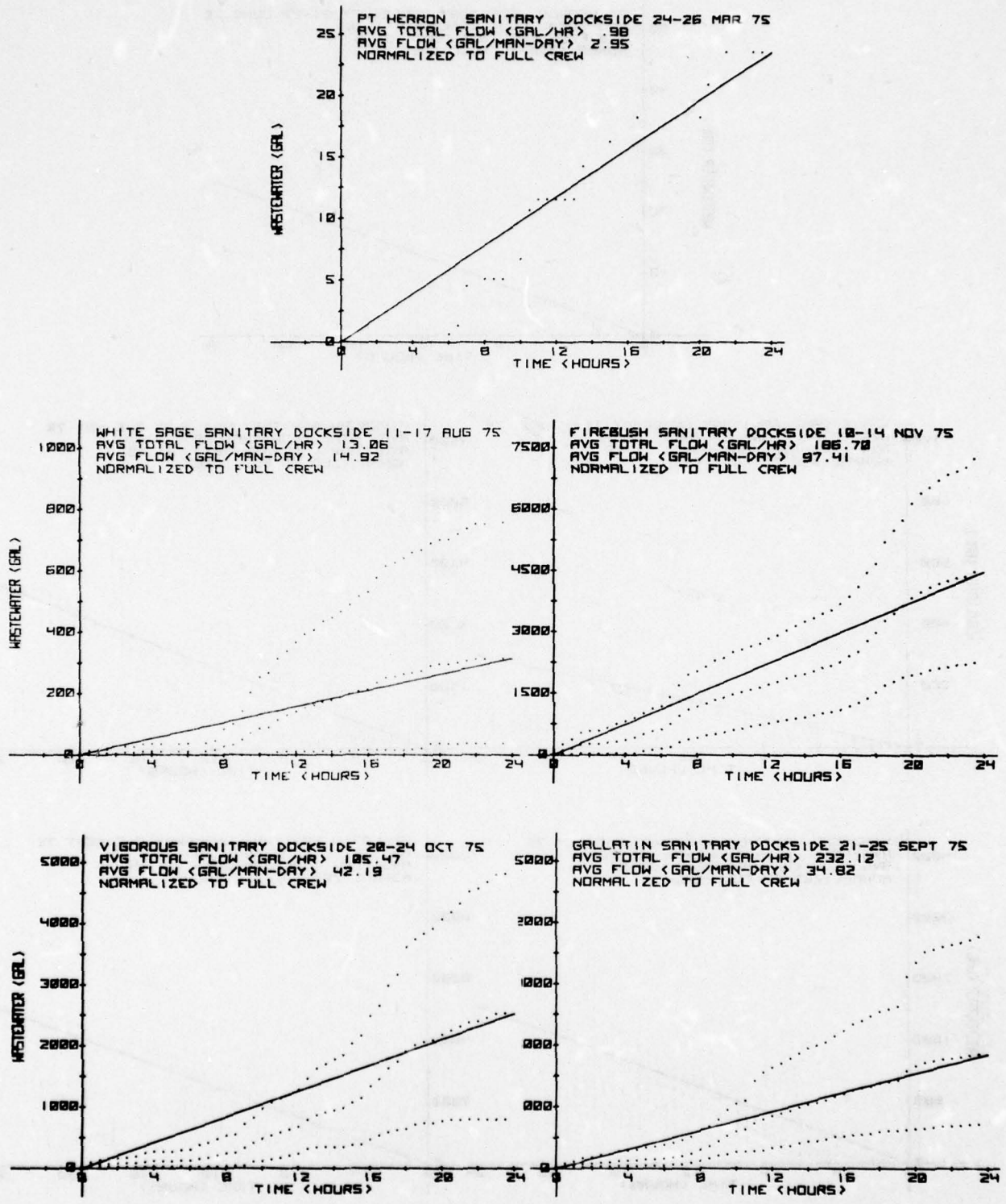
FIGURE 35. NORMALIZED SANITARY WASTEWATER FLOW; CUMULATIVE, DOCKSIDE
