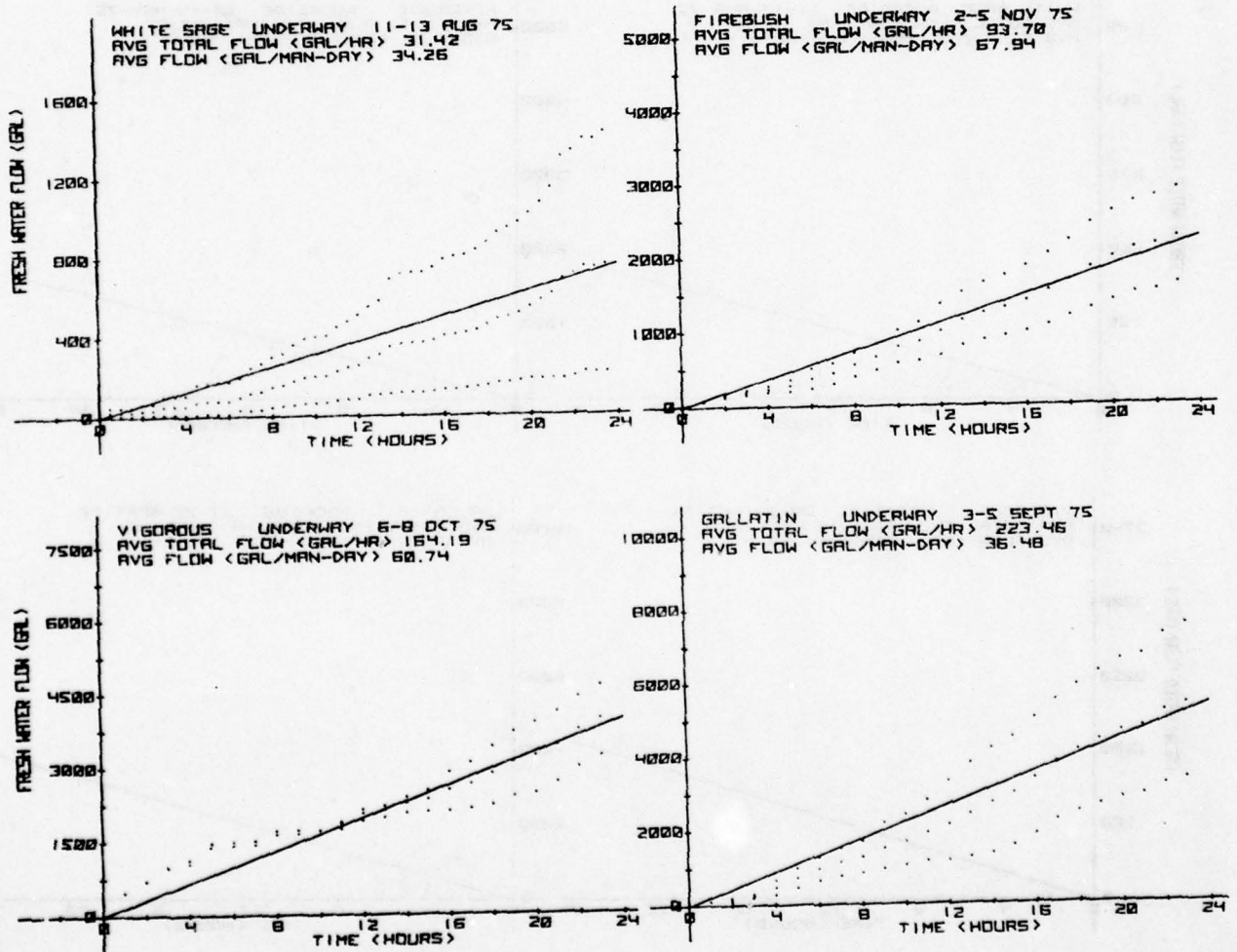
FIGURE 16. UNDERWAY CUMULATIVE FRESH WATER USAGE
