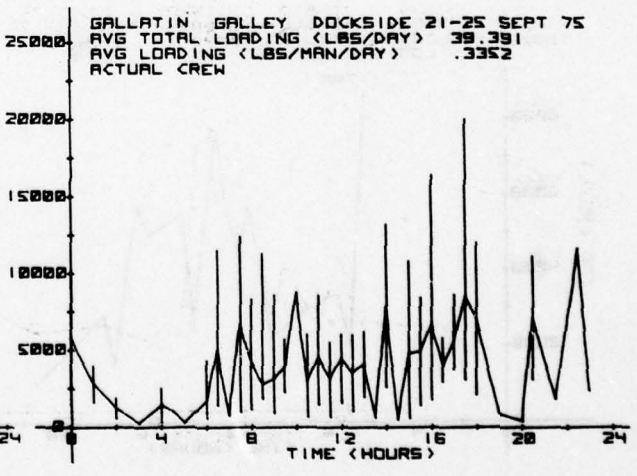
FIGURE 87. DOCKSIDE GALLEY COD LOADS
