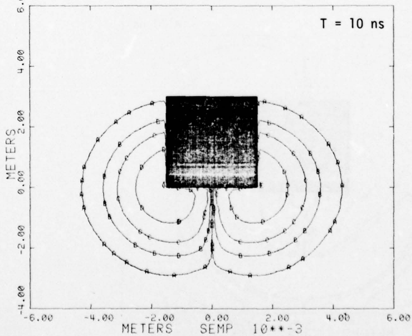
Figure 2.8. Contours of the magnetic field strength.
