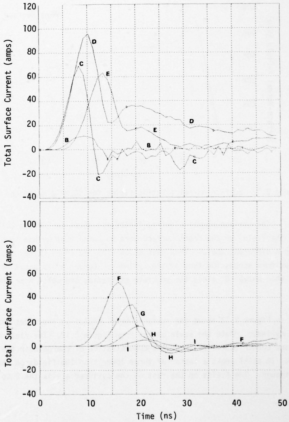
Figure 2.11. Total surface current for SGEMP simulation.
