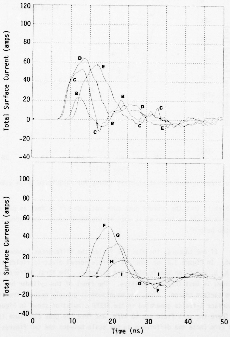
Figure 3.1. Total surface currents for capacitive drive simulation.
