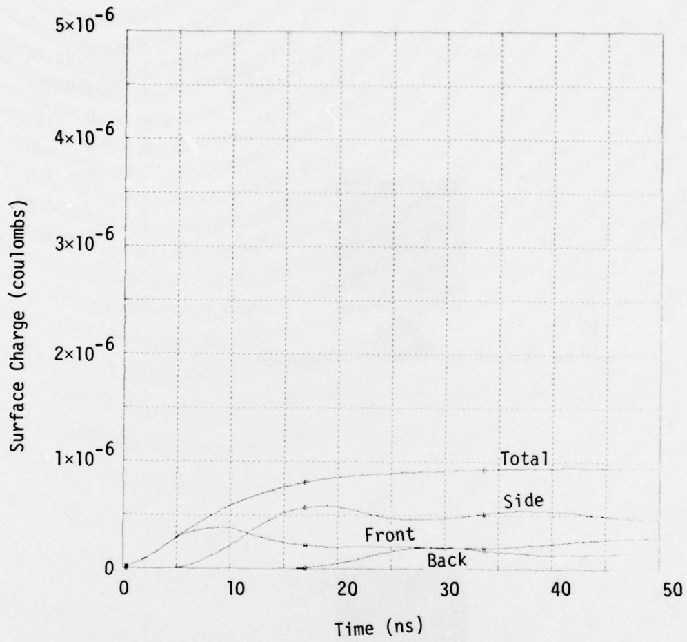
Figure 4.10. Charge on various surfaces of the cylinder for the direct drive simulation.
