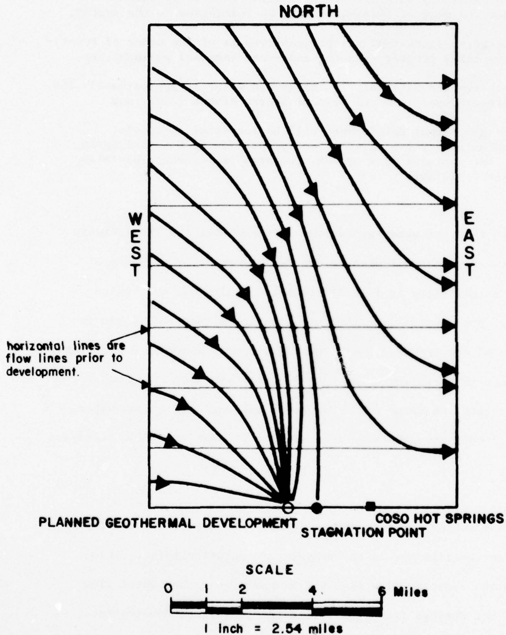
Figure 5. Plan View of Estimated Ground-Water Flow Lines in the Regional Flow System Prior to and Subsequent to Geothermal Development.
