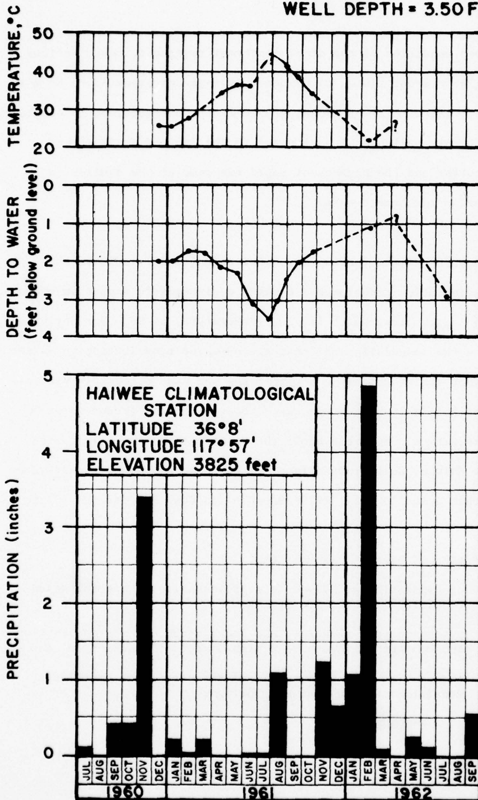
Figure 4. Relationship of Water Temperature and Ground-Water Depth at Coso Hot Springs, and Monthly Precipitation at Haiwee, California.
