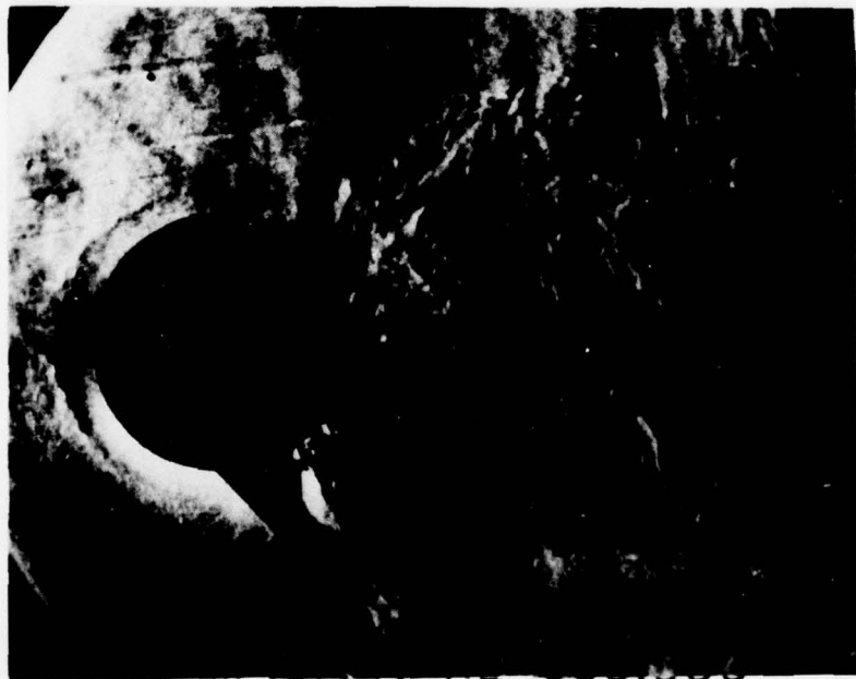
FLOW AROUND A TWO DIMENSIONAL CYLINDER AT THE CRITICAL MACH NUMBER (REF. 8)
