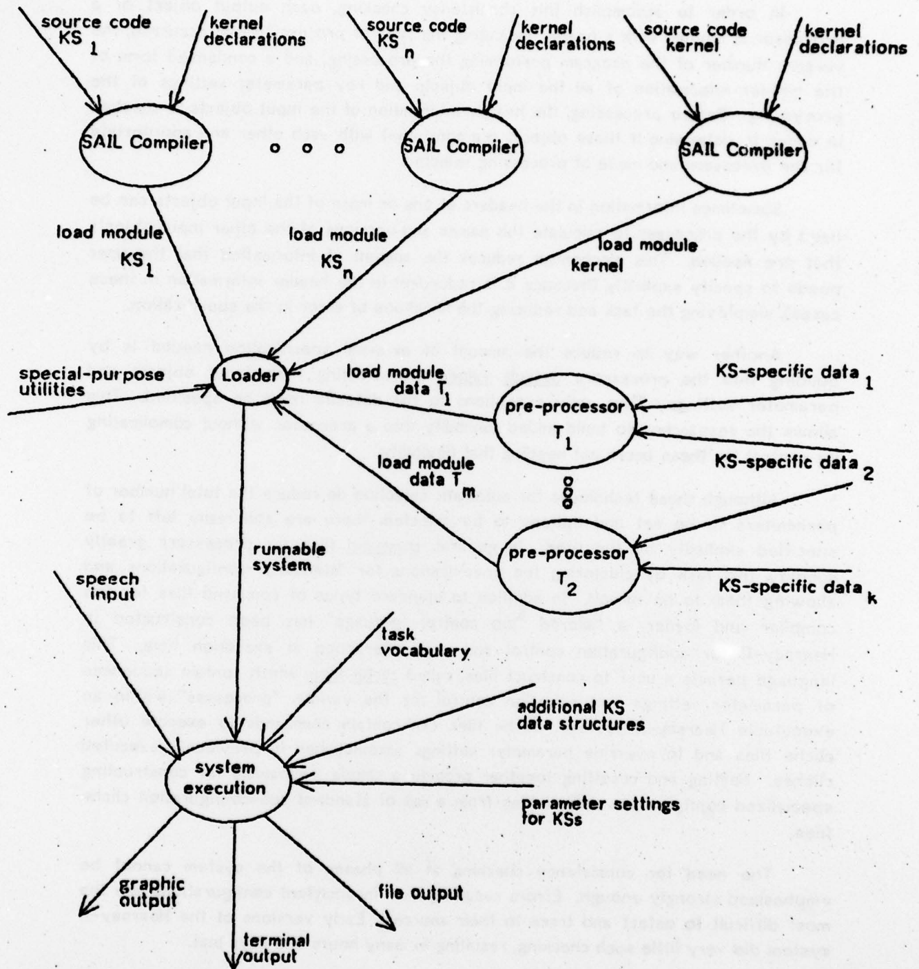
Figure 1: Creating and executing a Hearsay-II system (simplified).
