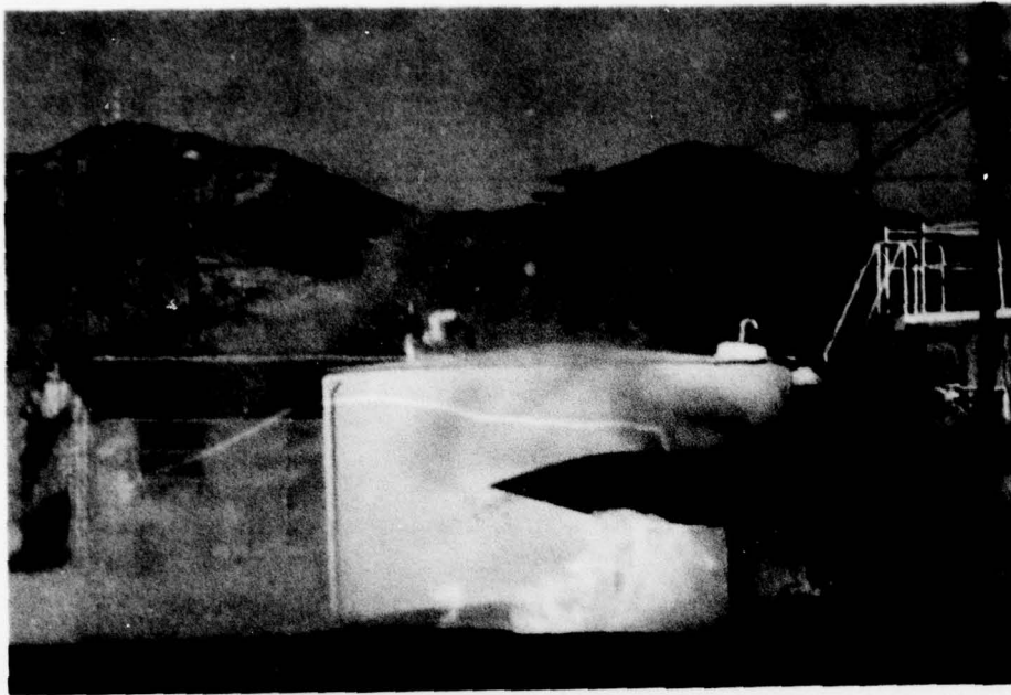
FIGURE 13. Flame propagation one-half second after torch ignition, test no. 41 (FM9 concentration - 0.35%, air velocity - 122 knots, fuel volume - 568 liters).
