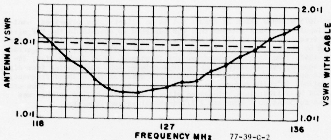
FIGURE C-2. FA-5675 ELLIPTICALLY POLARIZED (SWASTIKA) ANTENNA
