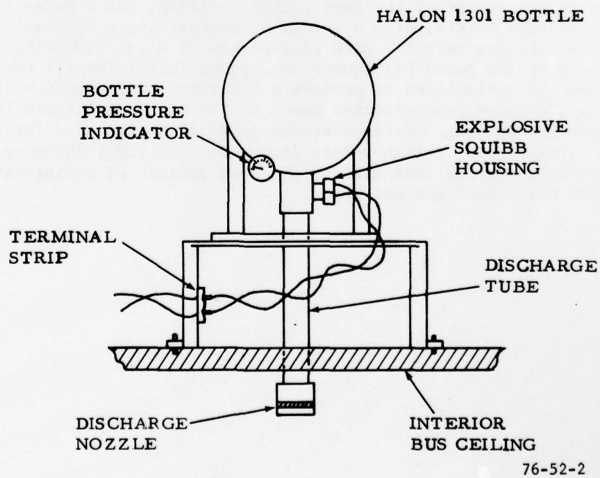
FIGURE 2. HALON 1301 BOTTLE INSTALLATION
