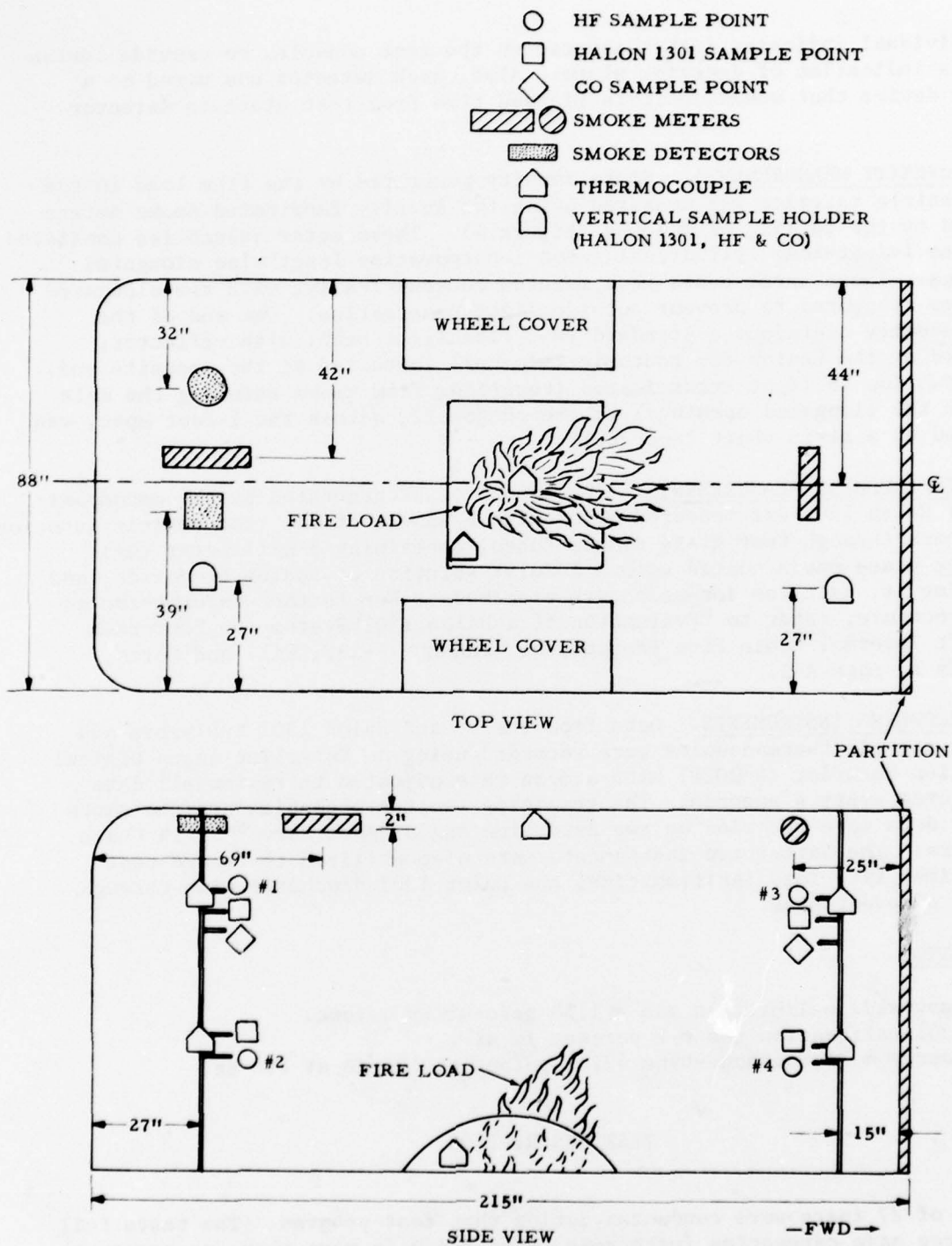
FIGURE 4. INSTRUMENTATION AND SAMPLE POINT LOCATIONS
