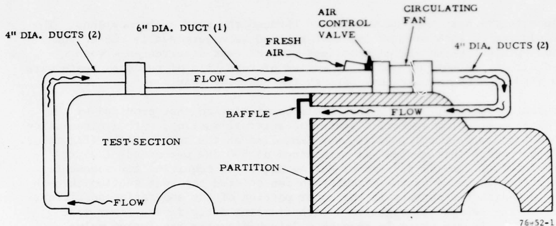
FIGURE 1. AIRFLOW-CIRCULATING SYSTEM
