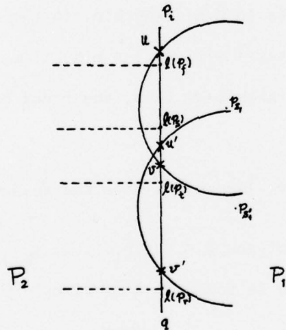
Figure 6. Illustration of the procedure in lemma 3.
