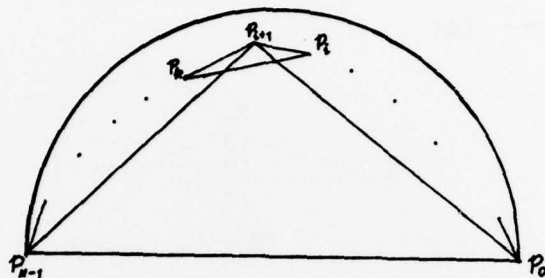
Figure 4. Illustration of the proof of lemma 2.
