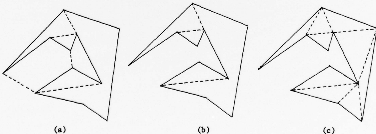
Figure 2. Simple polygon Q : (a) regularized; (b) decomposed into monotone polygons; (c) triangulated.
