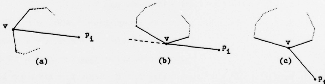
Figure 2. Illustration of convex, supporting, and reflex vertices.
