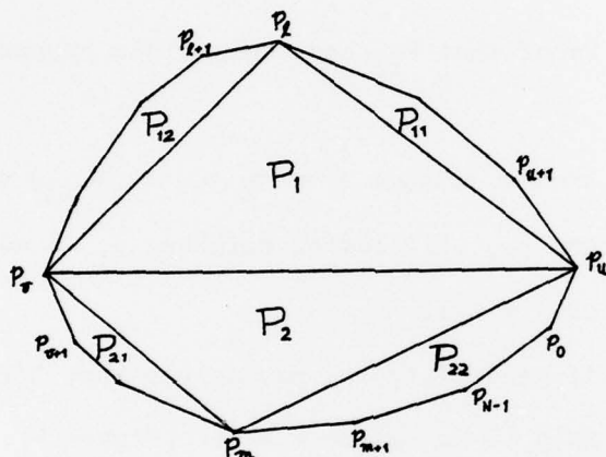
Figure 2. Decomposition of a convex polygon into four convex polygons satisfying semi-circle property.
