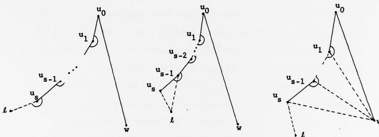
Figure 1. Triangulation of a monotone polygon.
