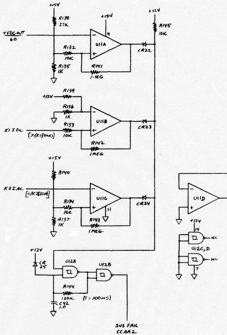
Figure 19 (Sheet 3 of 3). Converter Regulator and Control Schematic
