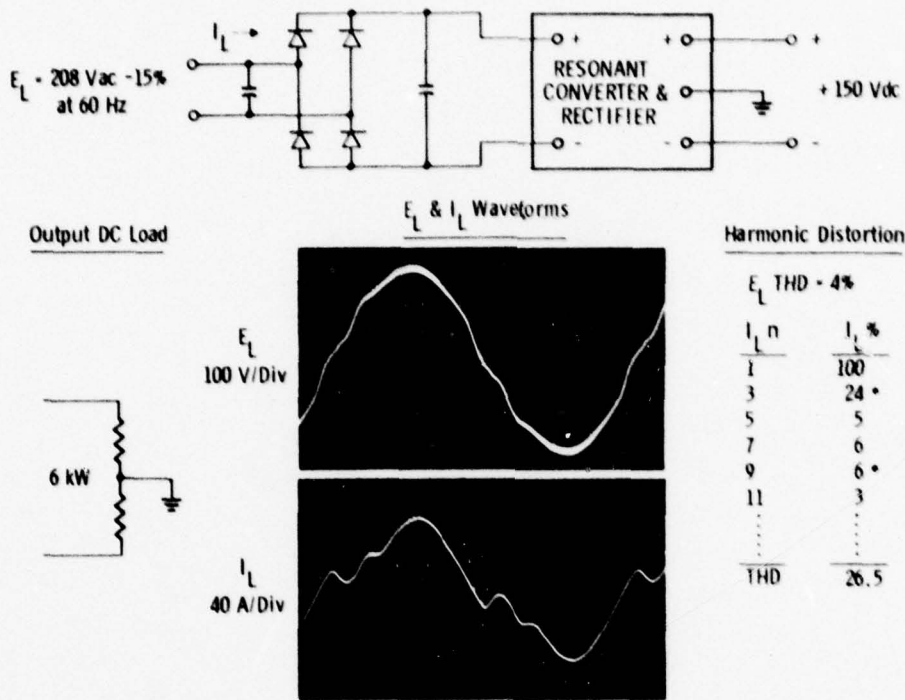
Figure 11. 1 \phi Converter Actual Performance
