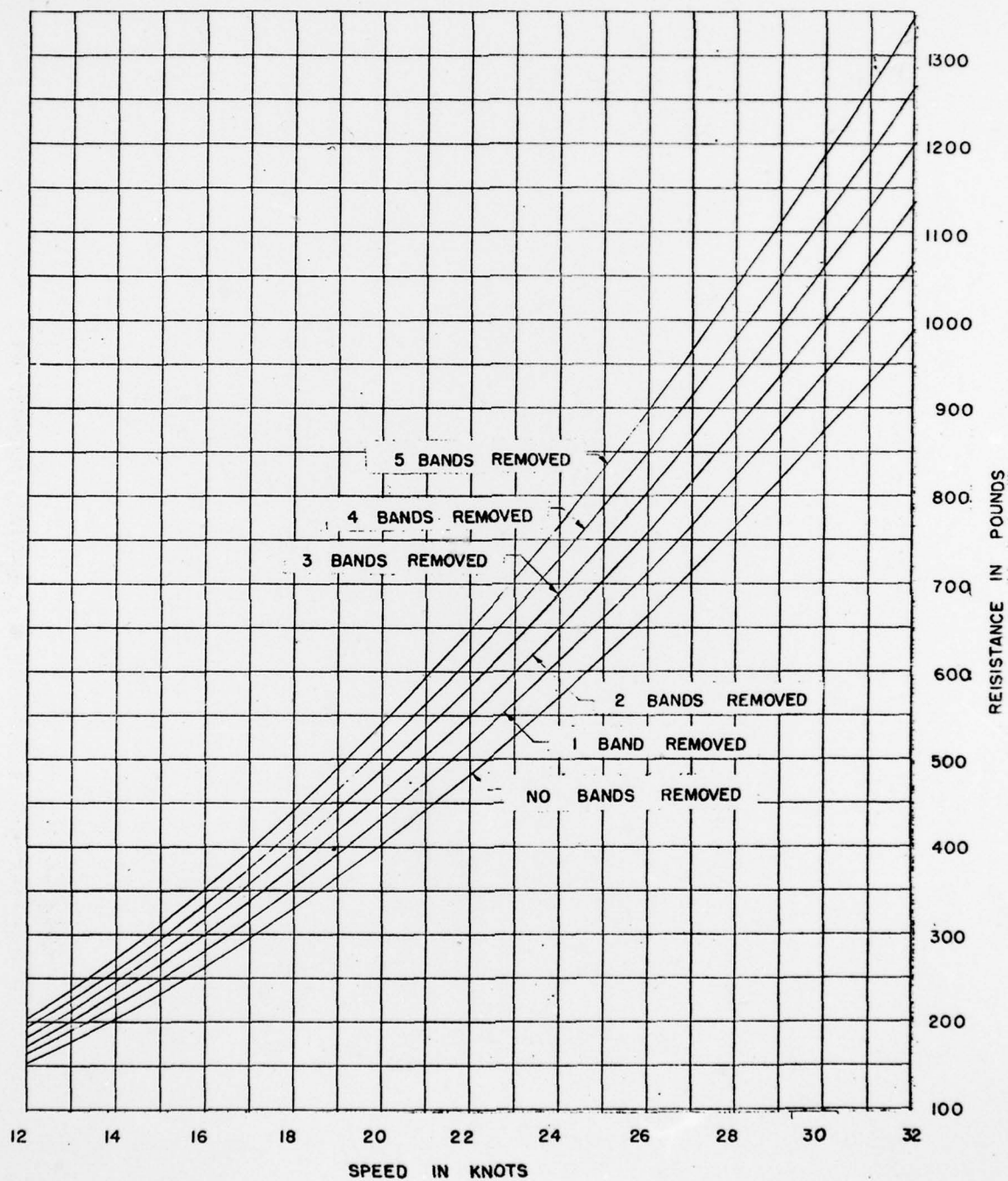
Figure 6 - Variation of Resistance Due to Removal of Cover Bands
