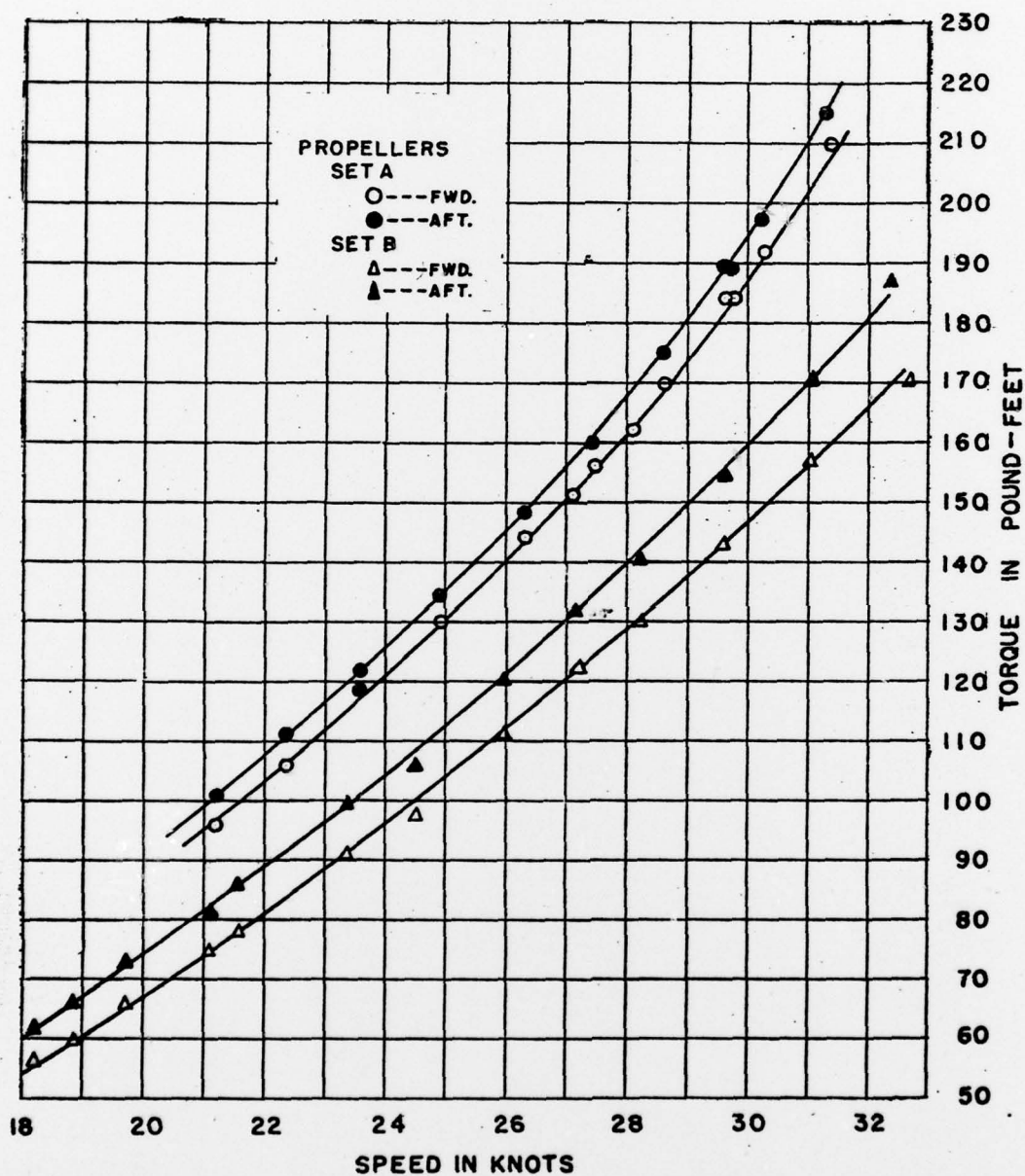
Figure 17 - Torque Unbalance for Propeller Sets A and B Installed on the 179-Inch Long Torpedo
