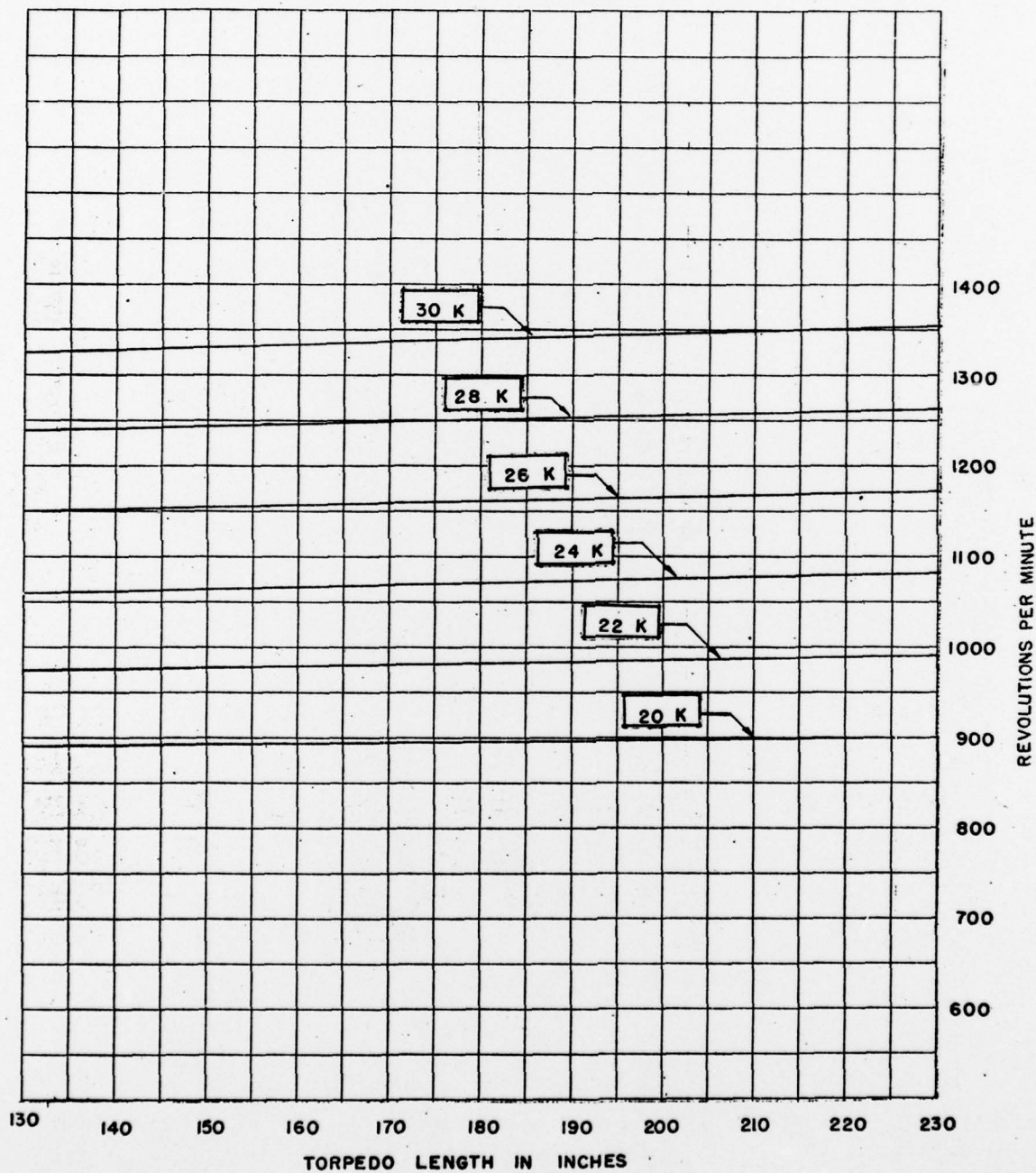
Figure 11 - RPM of the Various Torpedo Lengths with Propeller Set B
