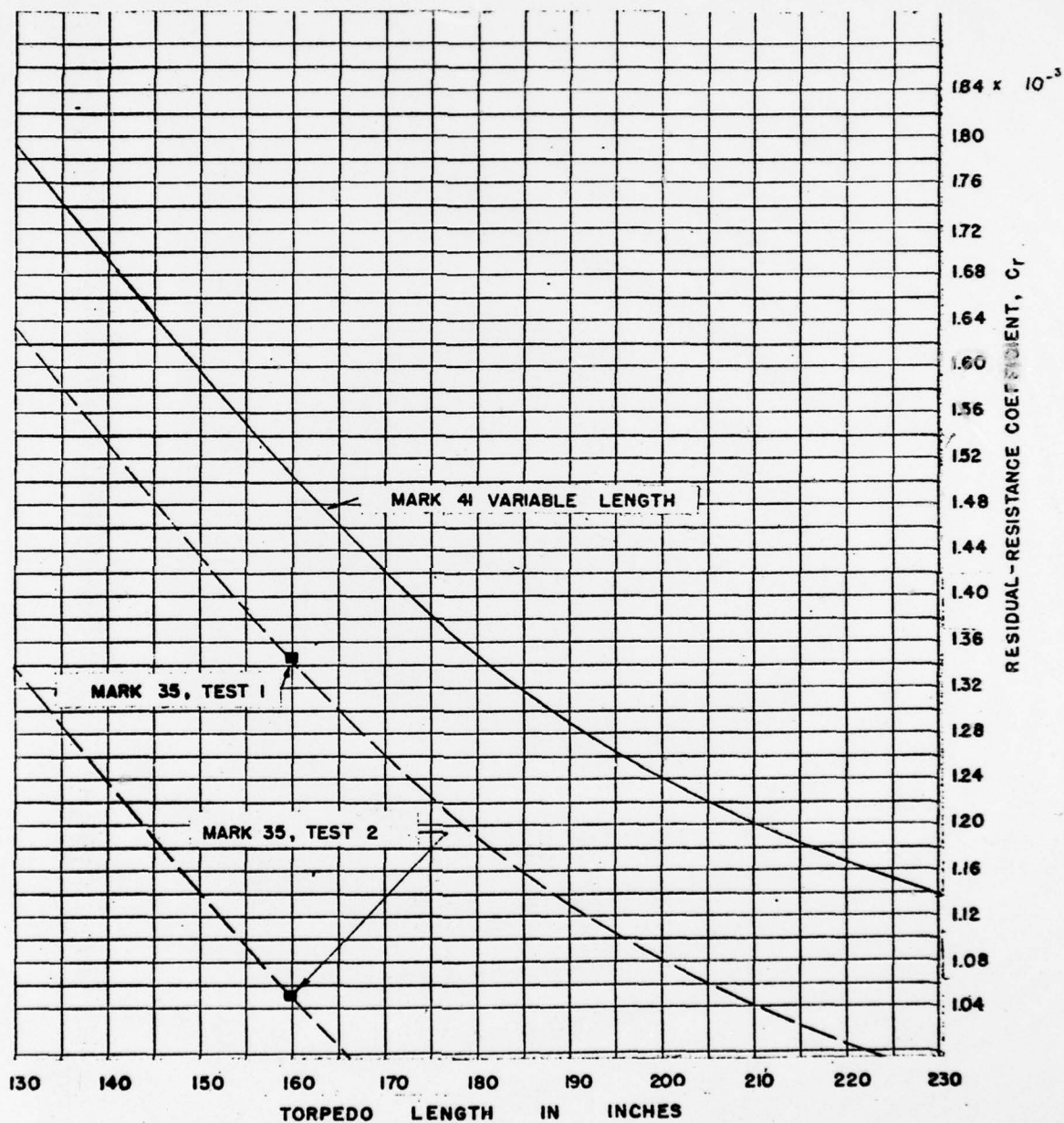
Figure 5 - Variation of C_r with Torpedo Length
