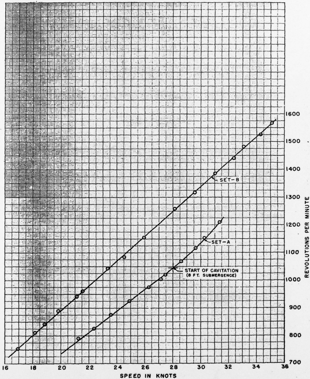
Figure 15 - RPM Versus Speed for the 179-Inch Length Torpedo
