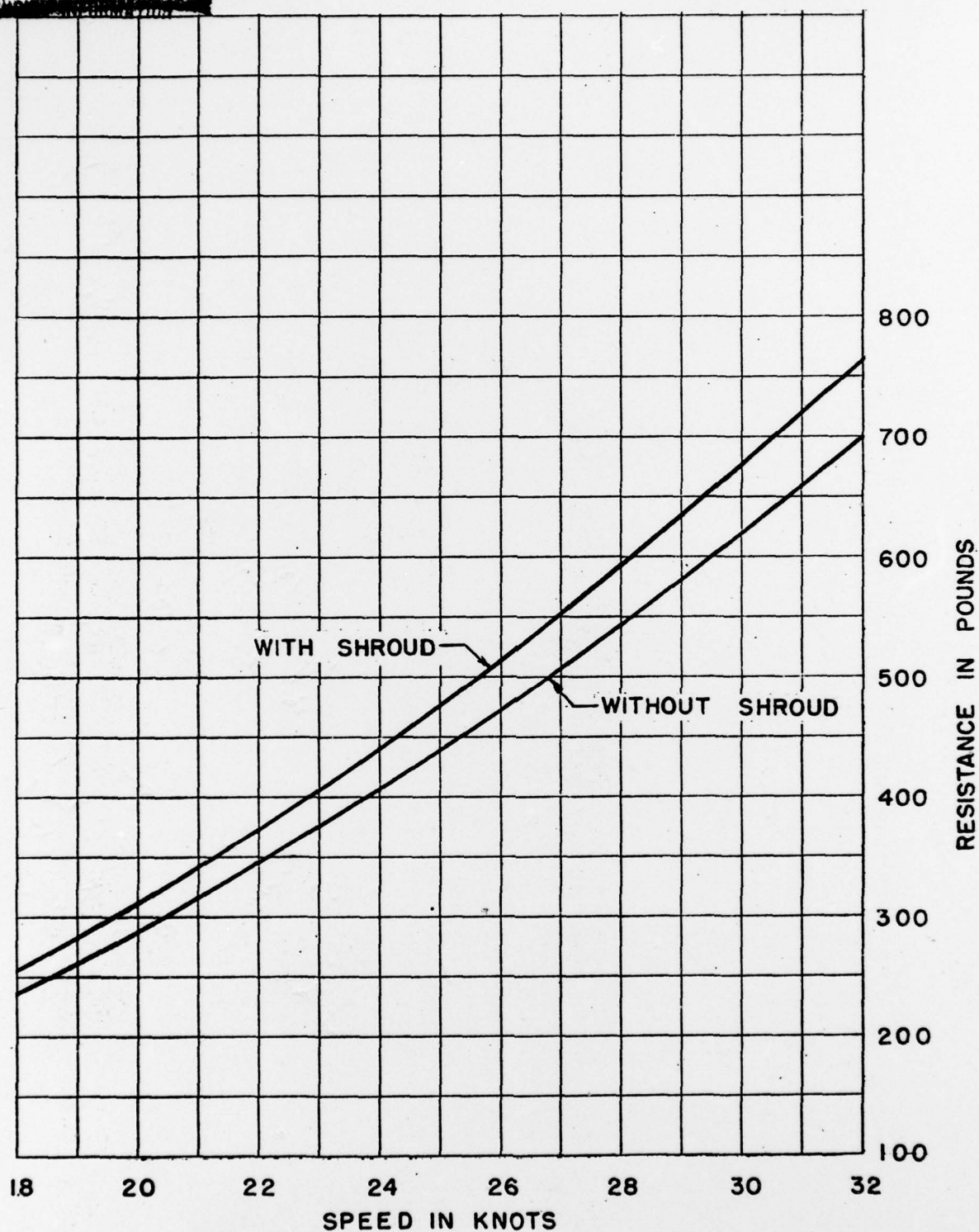
Figure 7 - Resistance Curves of the Torpedo with and without Shroud
