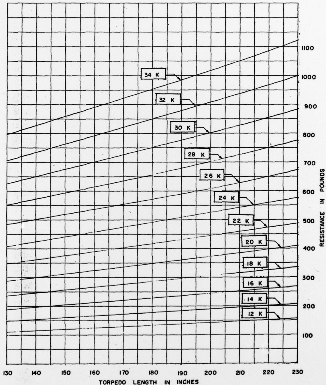
Figure 8 - Resistance of the Mark 41 Type Torpedo for Various Lengths
