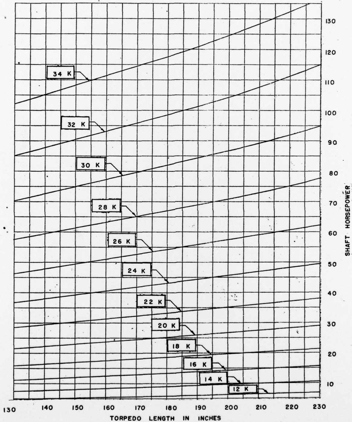
Figure 12 - Shaft Horsepower of the Various Torpedo Lengths with Propeller Set A
