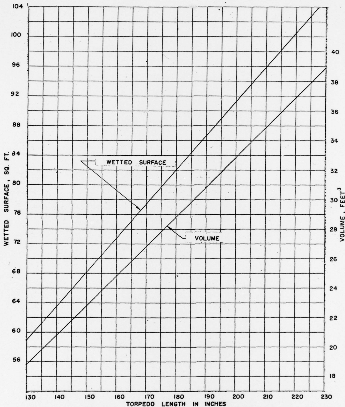
Figure 4 - Variation of Wetted Surface and Volume with Length Using the Nose, Afterbody and Control Surfaces of the Mark 41 Torpedo for the Basic Dimensions
