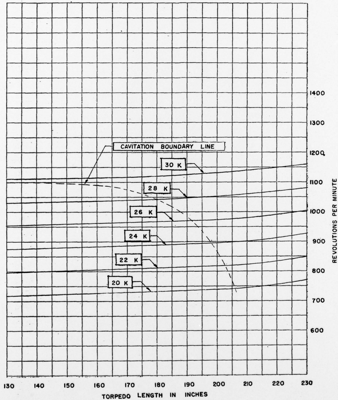
Figure 10 - RPM of the Various Torpedo Lengths with Propeller Set A
