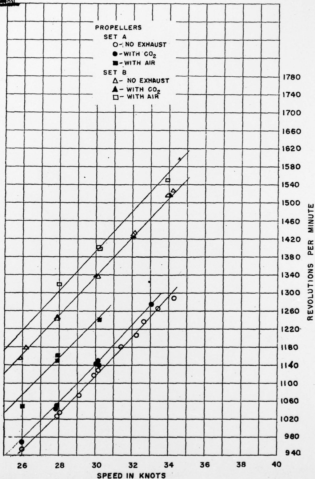
Figure 19 - Effect on the RPM of Exhausting Air or Carbon Dioxide into the Propeller Race
