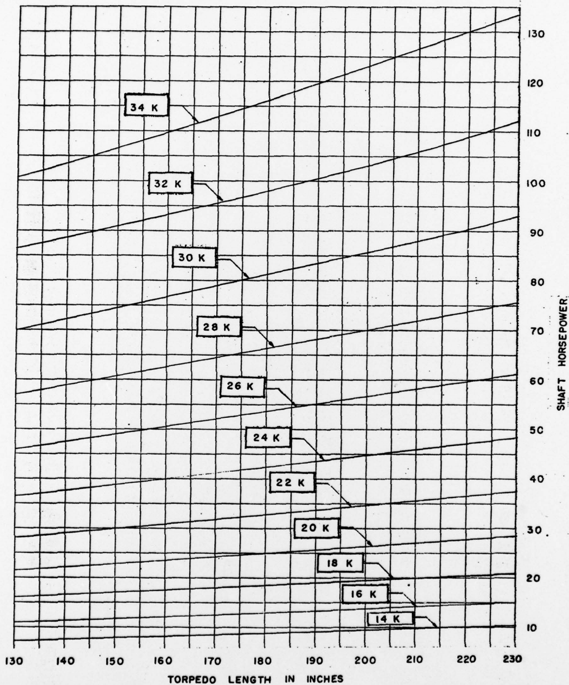
Figure 13 - Shaft Horsepower of the Various Torpedo Lengths with Propeller Set B
