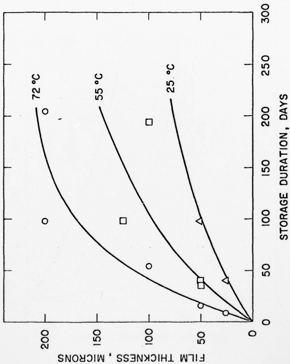
Fig. 34. L1 Film Growth on Storage in 1.0 (M) \text{LiAlCl}_4\text{-SOCl}_2 + 10% \text{S}_2\text{Cl}_2 (6wt%) at 72°, 55° and 25°C
