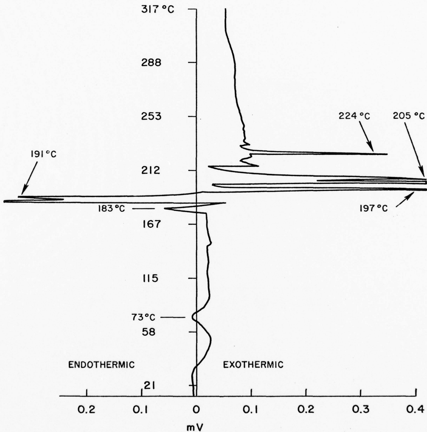
Fig. 78. Thermogram of \text{Li} + \text{S} + \text{S}_2\text{Cl}_2 , Sample #96
