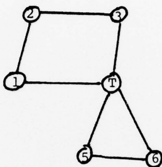
FIGURE 6. A FEASIBLE SOLUTION FOR d_i = 2
