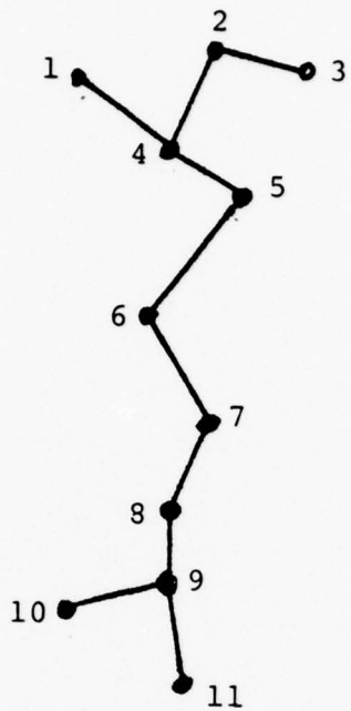
FIG 3. MINIMAL SPANNING TREE
