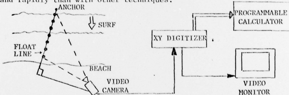
Figure 7 Video Surf Measurement and Analysis System
