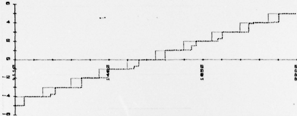
FIGURE 2. DIGITAL LED POSITION AND LR SCALED GTV CENTROID TRACK AZ OUTPUT VS TIME IN MSEC. 1 SD OF GTV LR- IS 1% OF FULL SCALE GTV OUTPUT LAG - 37.5 MSEC
