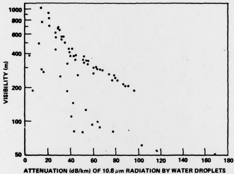
FIG. 6. PLOT OF VISIBILITY VERSUS ATTENUATION AT 10.6- \mu\text{m}
