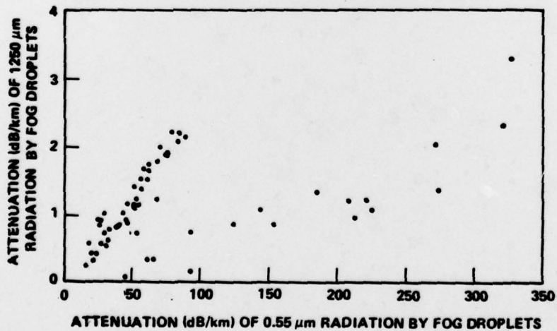
FIG. 7. COMPARISON OF ATTENUATIONS OF 1250- \mu\text{m} AND 0.55- \mu\text{m} WAVELENGTHS BY FOG DROPLETS
