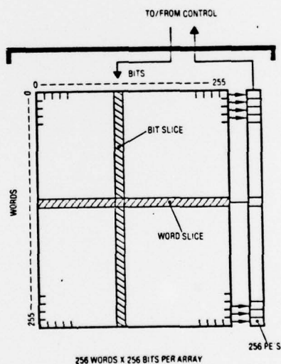
Figure 2. Associative array
