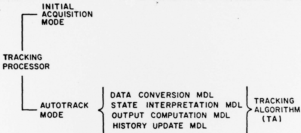
FIGURE 4. TRACKER PROCESSOR FUNCTIONS
