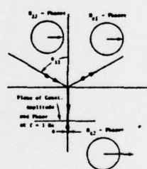
Figure 4 Reflection-transmission geometry for Air in Seawater
