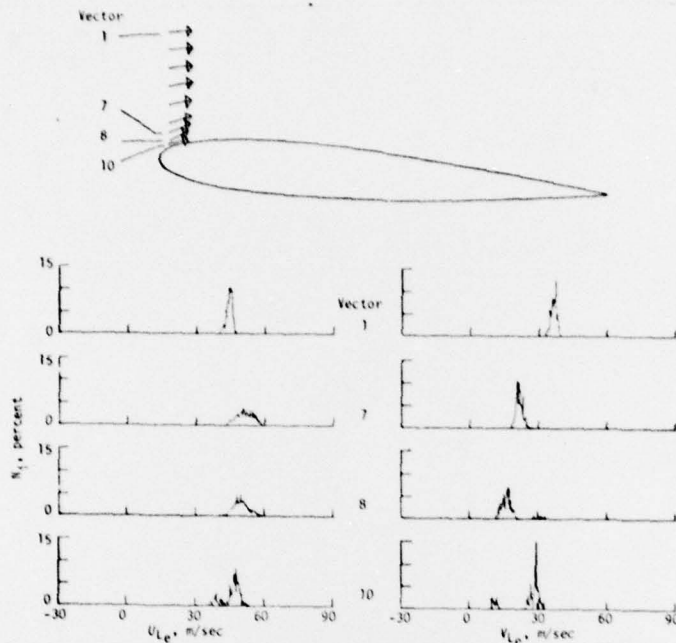
Figure 9. - Histogram data for scan C. Wing geometric angle of attack = 4.15^\circ .
