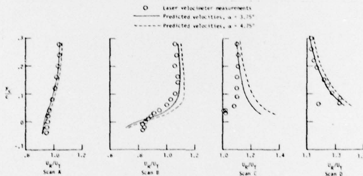
Figure 8. - Comparison of LV flow-field velocity measurements with a two-dimensional viscous-flow prediction. Wing geometric angle of attack = 4.15^\circ .
