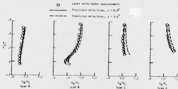
Figure 6. - Comparison of LV flow-field velocity measurements with a two-dimensional viscous-flow prediction. Wing geometric angle of attack = 0^\circ .
