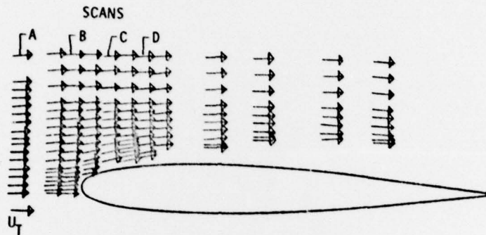
Figure 5. - Velocity vectors computed from measurements over the wing at a geometric angle of attack of 0^\circ .
