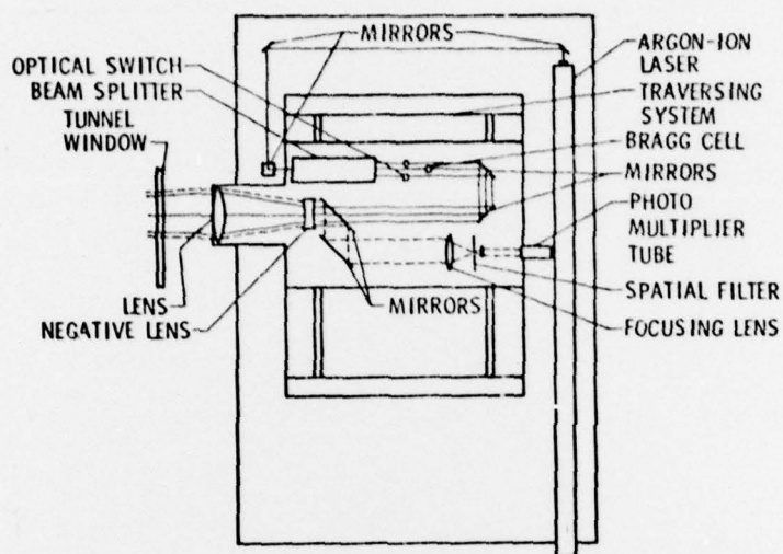
Figure 2. - Schematic of the LV optics.
