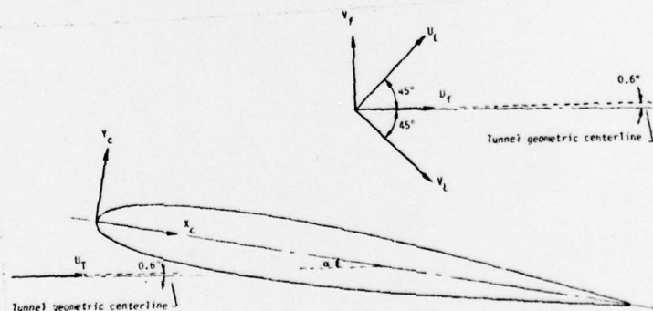
Figure 1. - Sketch of axis system used including directions of velocity components computed.
