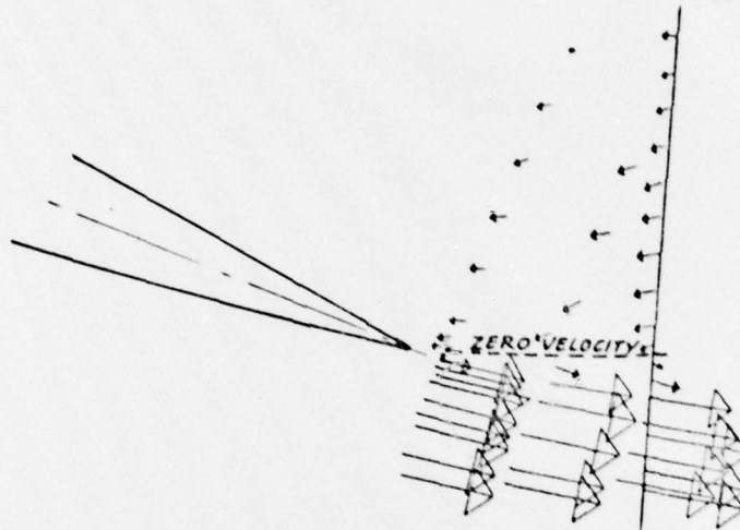
Figure 11. - Velocity measurements at the trailing edge of the wing at \alpha = 19.4^\circ .
