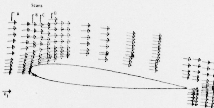
Figure 7. - Velocity vectors computed from measurements over the wing. Geometric angle of attack = 4.15^\circ .
