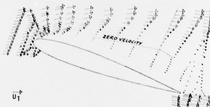
Figure 10. - Velocity measurements over the stalled wing ( \alpha = 19.4^\circ ).
