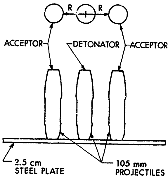
Figure 1. Schematic of typical test configuration for interround communication
