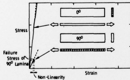
Figure 1a. Schematic diagram of tensile stress-strain curves of a 0^\circ lamina, a 90^\circ lamina and a 90/0/90^\circ laminate.
