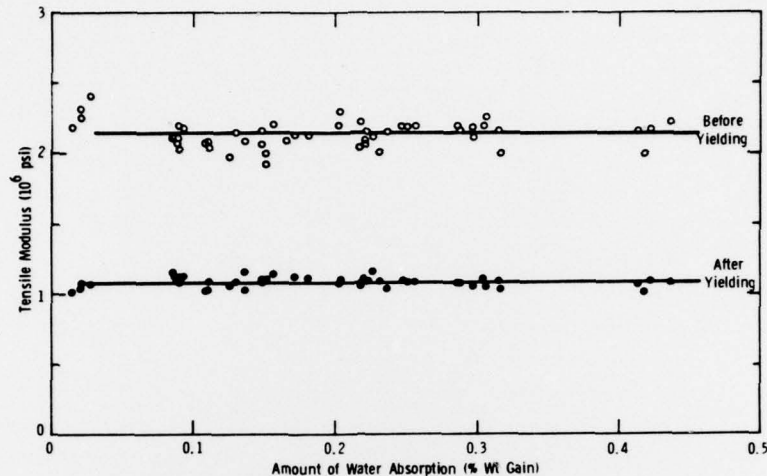
Figure 5. Effect of water absorption on the tensile modulus of a 90/0/90° laminate.
