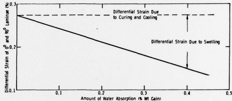
Figure 8. Effect of water absorption on the calculated differential strain of 0^\circ and 90^\circ laminae.
