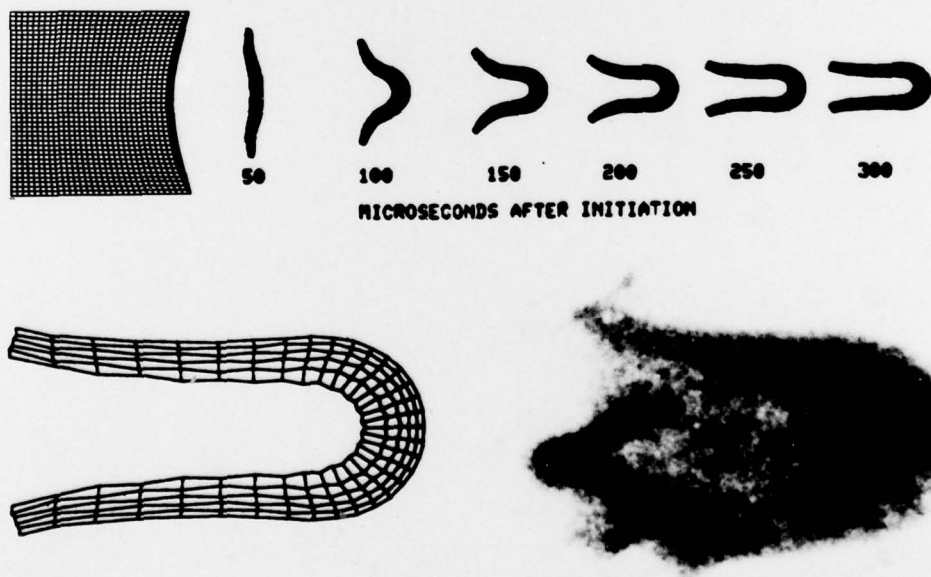
Fig 3 HEMP solution for Kronman's ballistic disc and flash x-ray of fragment
