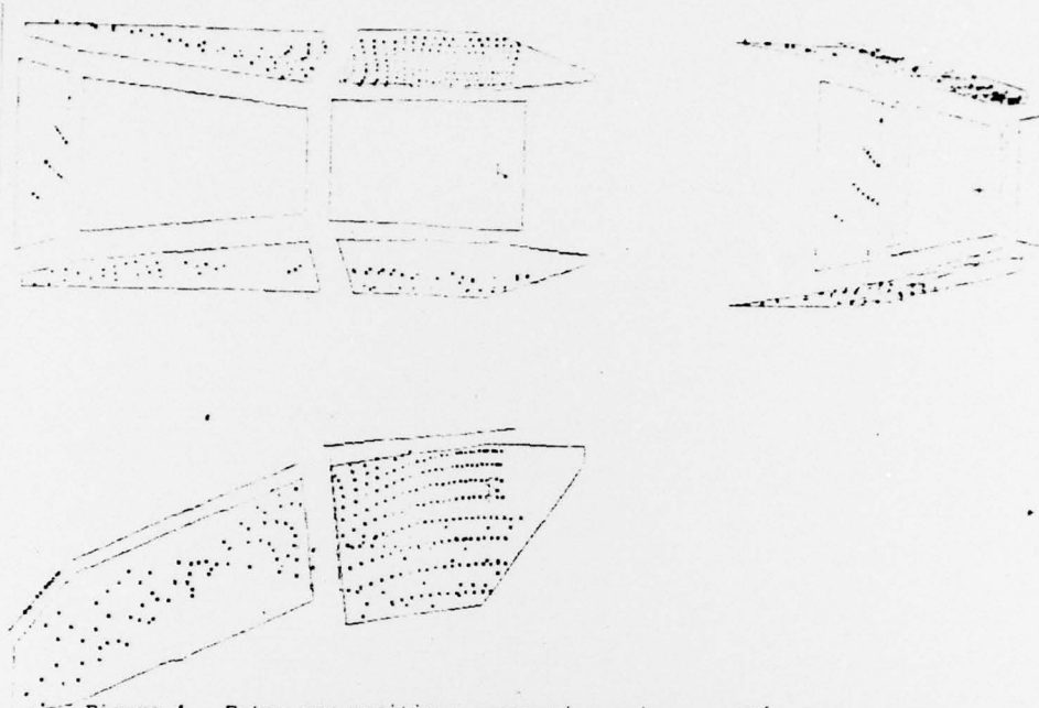
Figure 4. Entry ray positions generating primary reflections on the right-hand side of the canopy as seen from the pilot's position.
