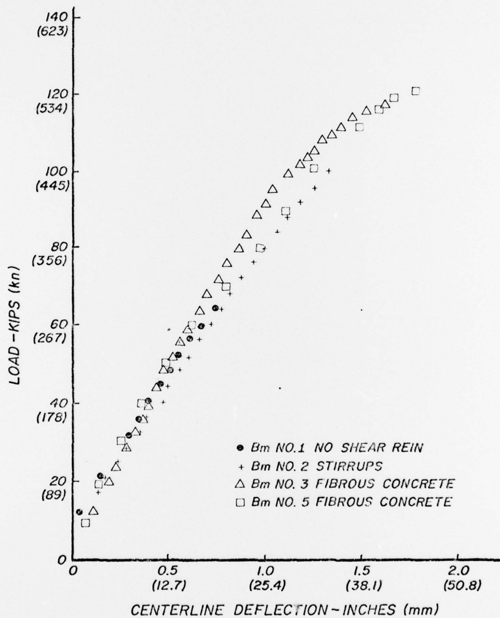
FIG. 6 LOAD-DEFLECTION CURVES
