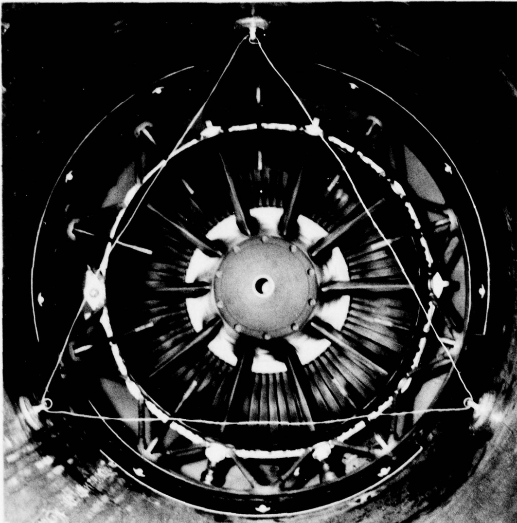
Figure 6. The TRION grid probe and PRION probe as viewed from the end of the tailpipe on a TFW1 engine. Each side of the triangle probe is 2 ft long.
