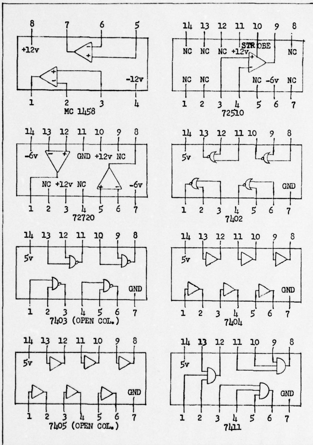
Figure A-11. IC's used in the Wear Rate Monitor, except A-8400 voltage-to-frequency converter. (Continued next page)
