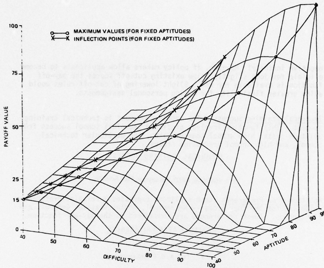
Figure 8. Pay-Off Function of Aptitude and Difficulty.
