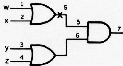
Figure 2.1a. Single fault: line 5 stuck-at value s , s \in (0,1)
