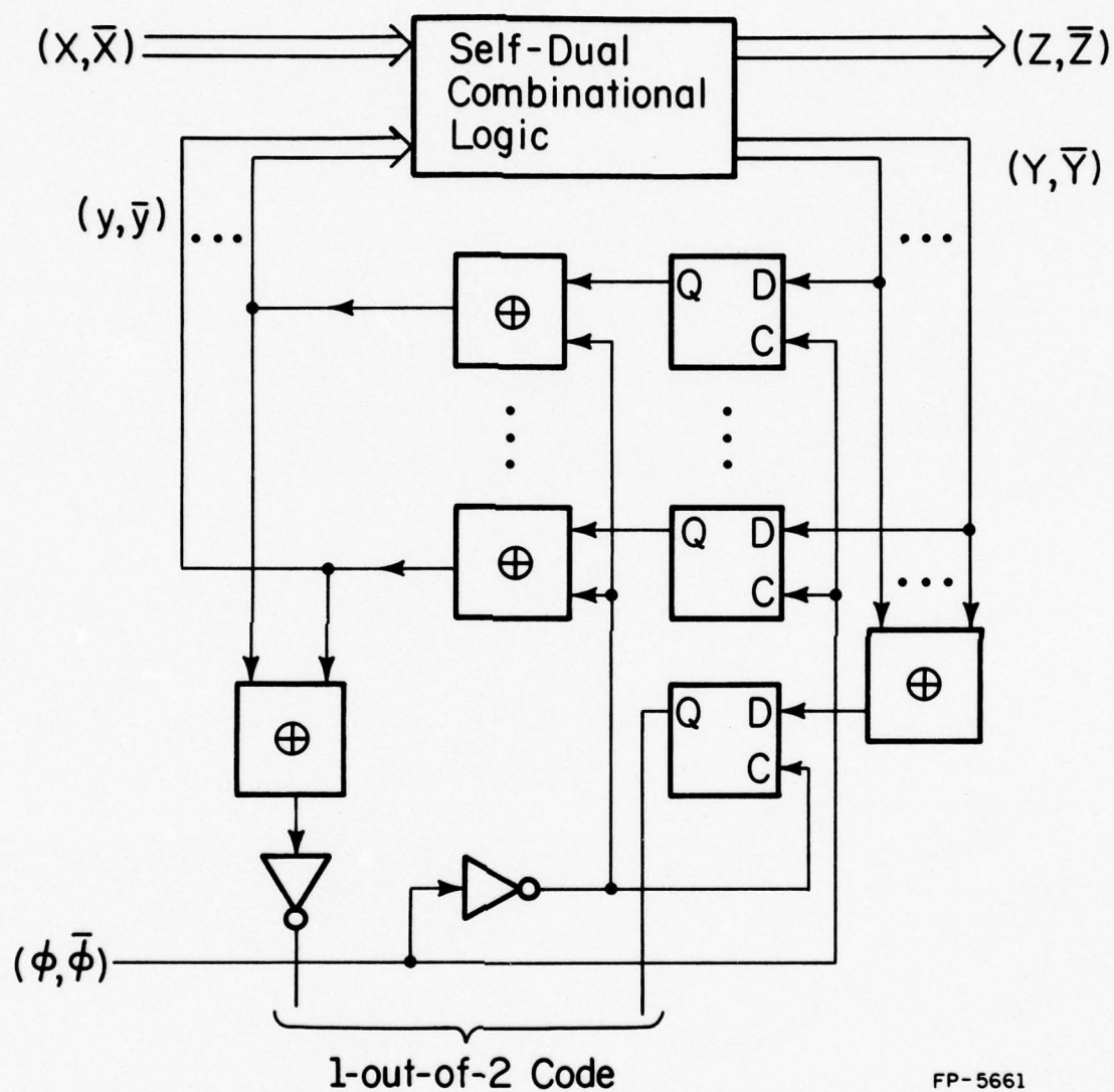
Figure 4.5. Complete code translation system
