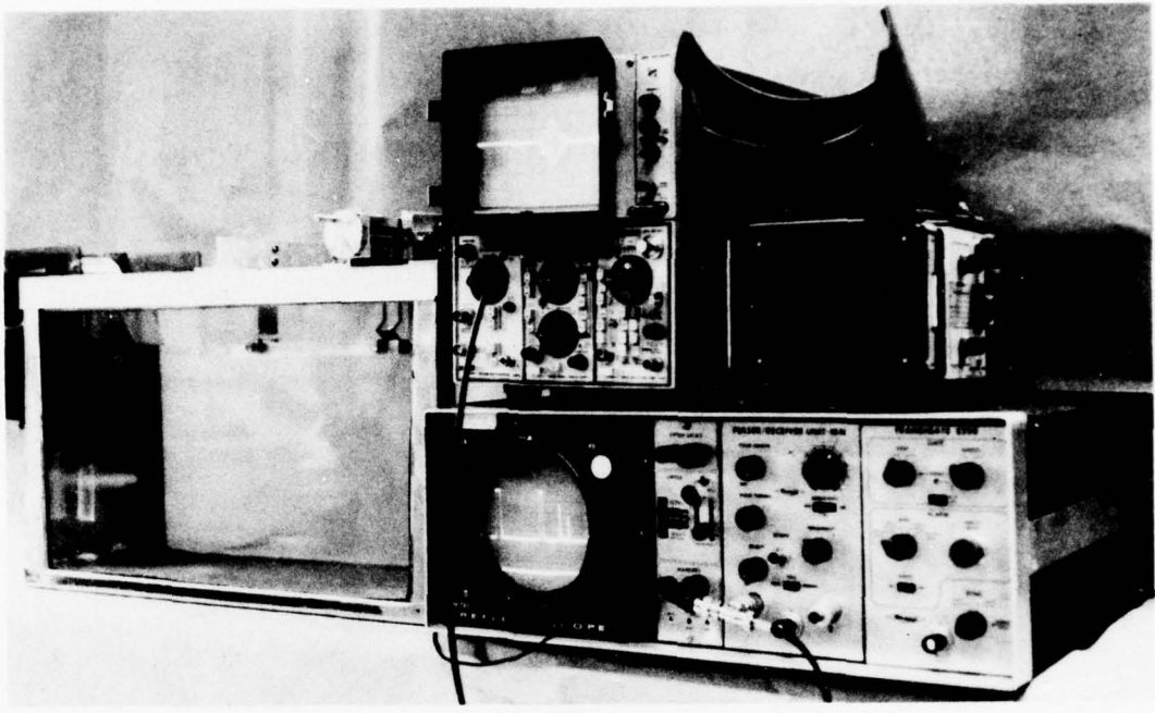
a. Water Immersion Tank and Test Equipment
