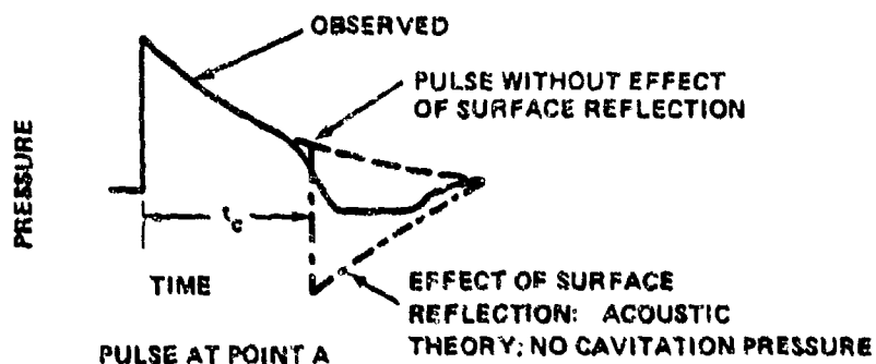
FIG. 7 TYPICAL PRESSURE PULSES AFFECTED BY SURFACE REFLECTION
