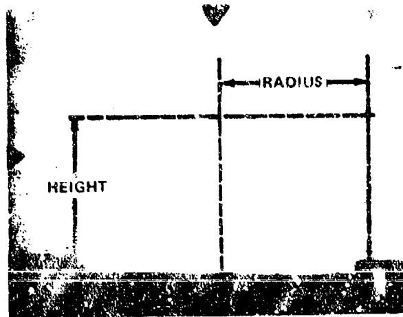
FIG. 14-1 PLUME DIMENSIONS
