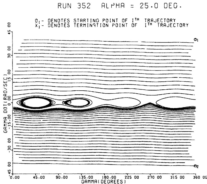
Figure 8. Rolling Motion Phase Plane for Body Plus Tail Configuration at a 25° Angle of Attack
