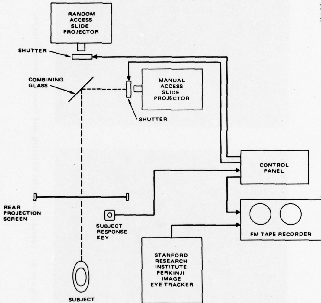
Figure 9. Schematic diagram of experimental apparatus.
