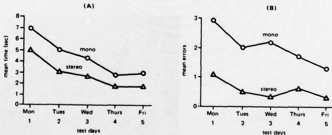
Figure 3. Mono vs stereo link task time scores (A), and error scores (B) with repeated testing.
