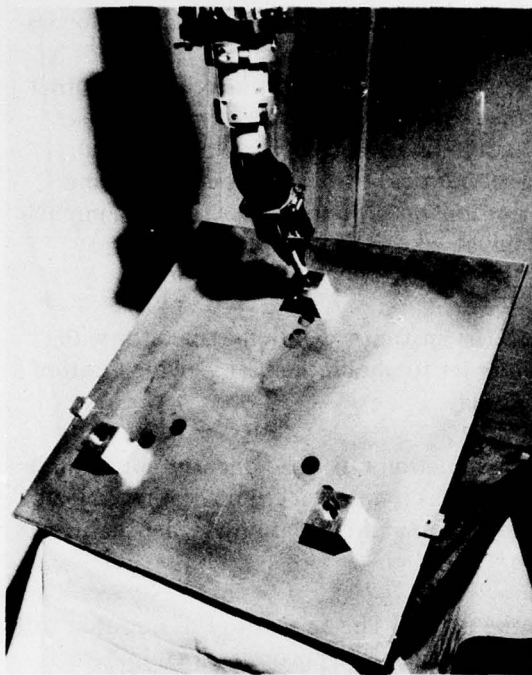
Figure 1. Peg-in-hole alignment taskboard.
