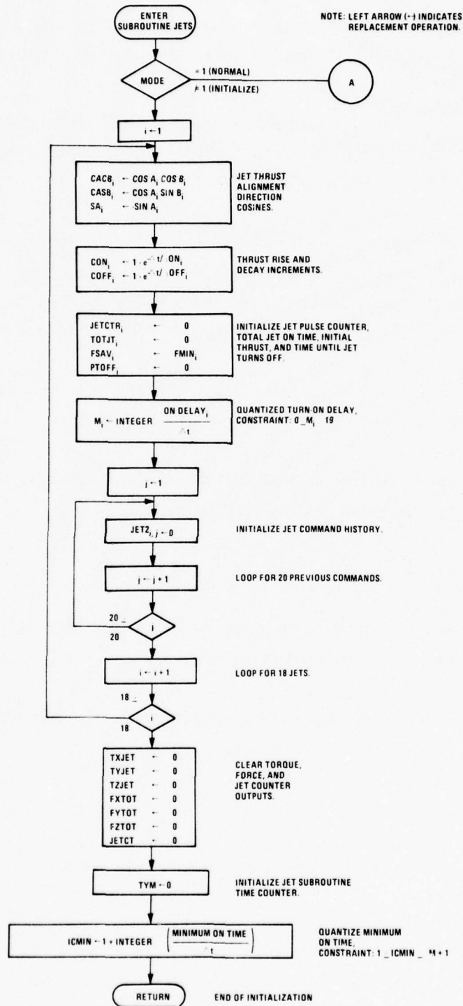
Figure F-1. Flow Diagram of Reaction Jet Model
