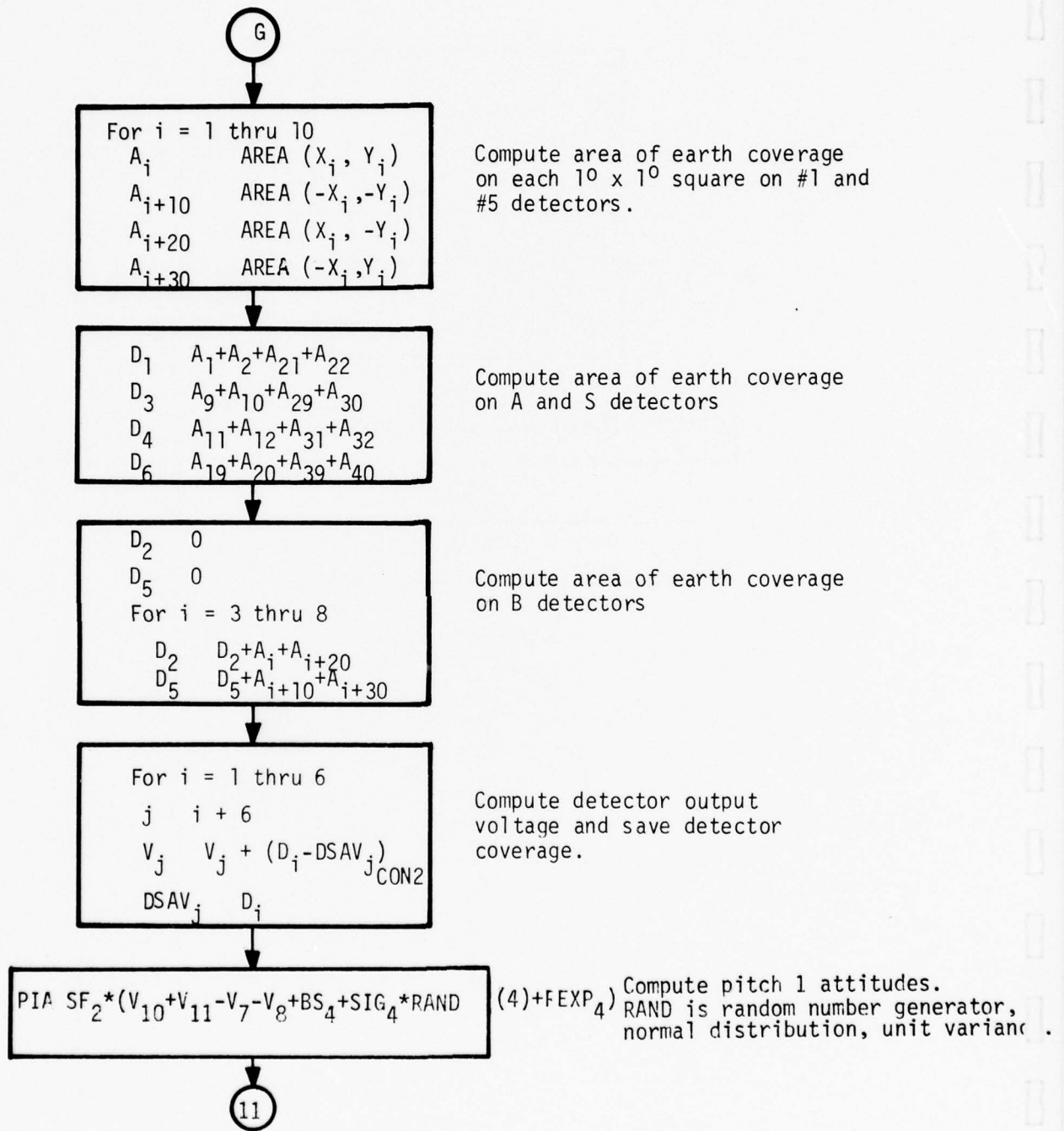
FigureJ-6. Earth Sensor Flow Chart (continued)
