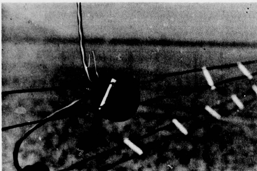
Figure 5 New switch. Components are totally encapsulated in opaque epoxy. Switch leads are protected inside cable jacket.
