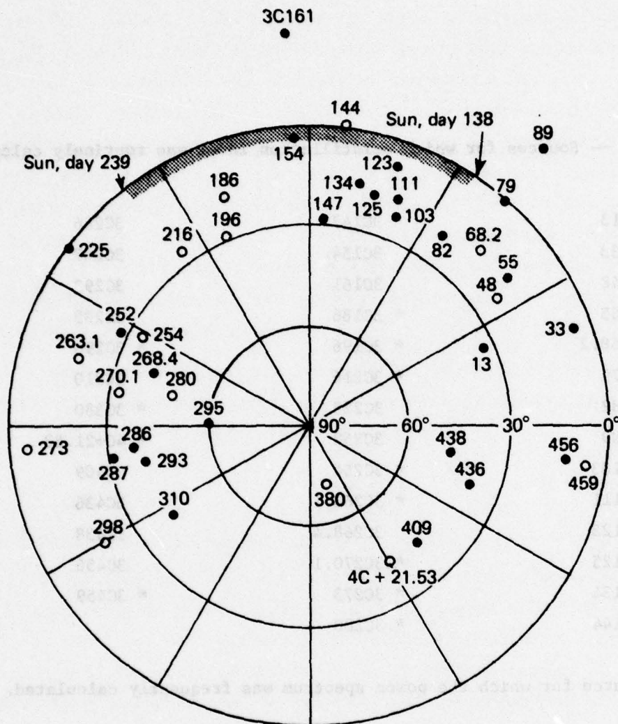
Fig. 1 Subset of 41 sources observed by the COCOA-Cross radio telescope. Sources plotted with an open circle consistently yielded useful spectra.
