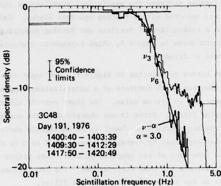
Fig. 8 Power spectrum of the scintillating radio source 3C48 on 1976, day 191.
