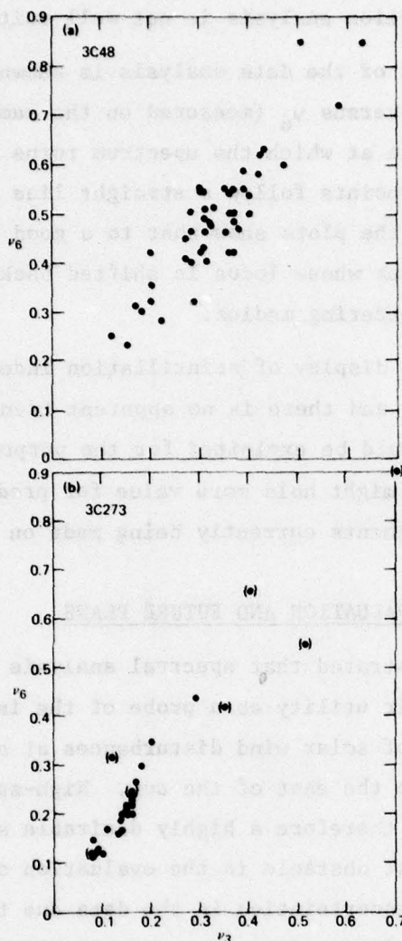
Fig. 12 Scatter plots of \nu_3 versus \nu_6 for 3C48(a) and 3C273(b). The high correlation between these two parameters implies a consistently similar shape for the spectra, i.e., a universal curve which shifts on the frequency axis in response to solar wind velocity and turbulence profile. The closer grouping of the 3C273 points may be due in part to large source angular diameter effects. The points in parenthesis for 3C273 are taken from 2 component spectra, which result from two widely separated scattering regions in the interplanetary medium.
