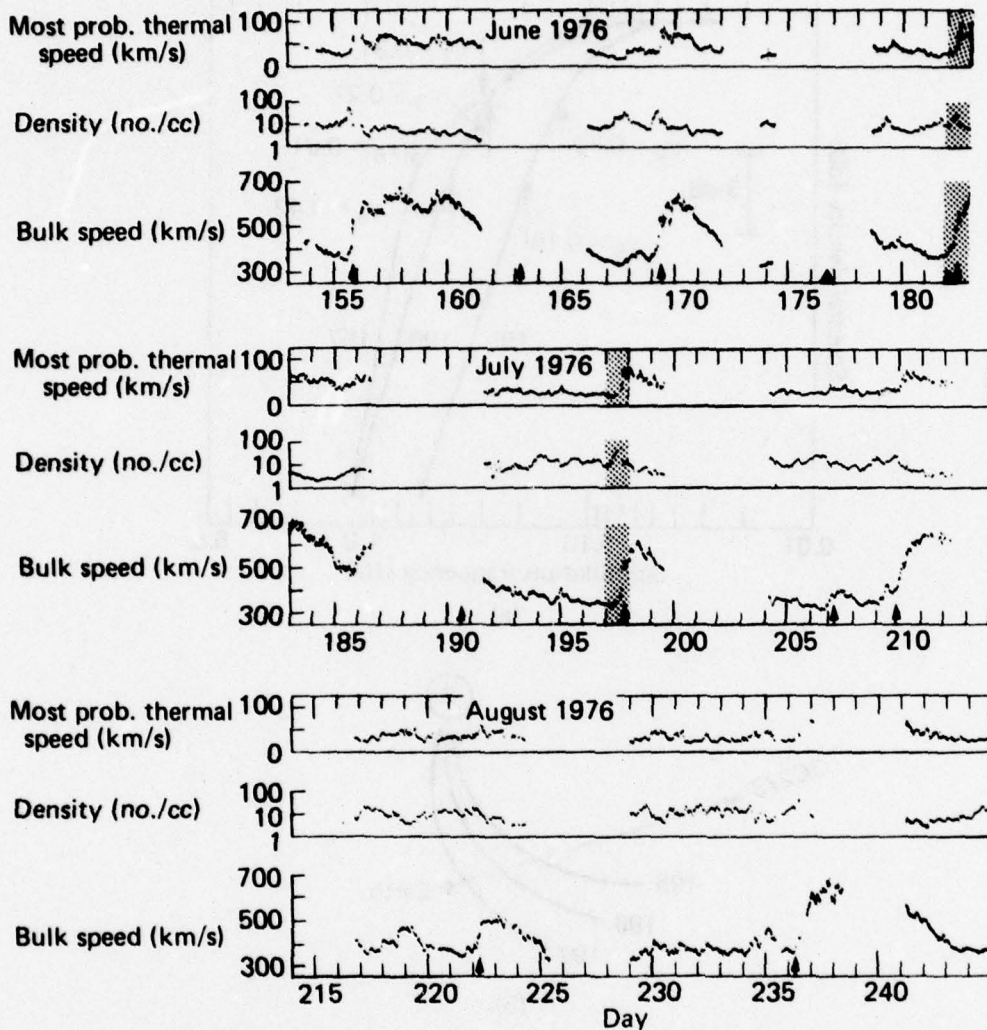
Fig. 10 Solar wind probe data (Lazarus, Solar-Geophysical Data , 1977), days 153-244, showing recurring corotating solar wind streams. Shaded areas correspond to known streams with sufficient IPS data coverage to be used in the prediction study. Triangles are geomagnetic sudden commencements; arrows are abrupt increases in K_p index.
