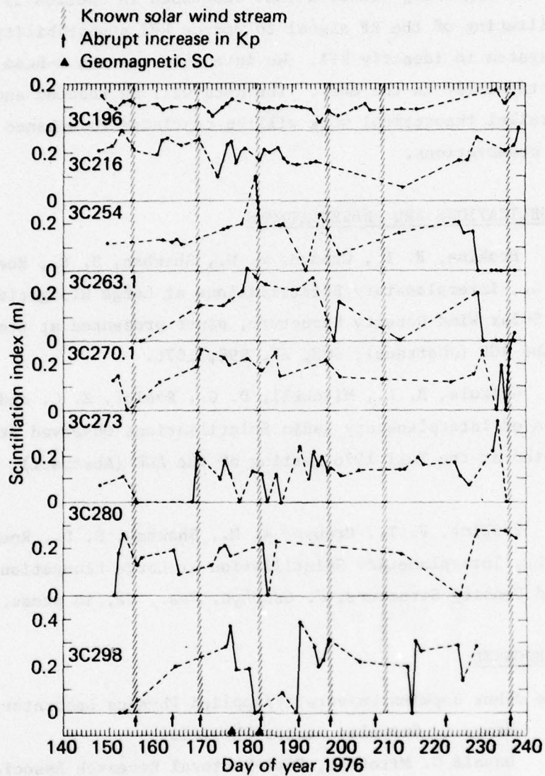
Fig. 13 Scintillation index versus time for 8 eastern sources. The shaded regions indicate the density enhancements preceding several high speed solar wind streams. Abrupt increases in K_p and geomagnetic sudden commencements are also indicated.
