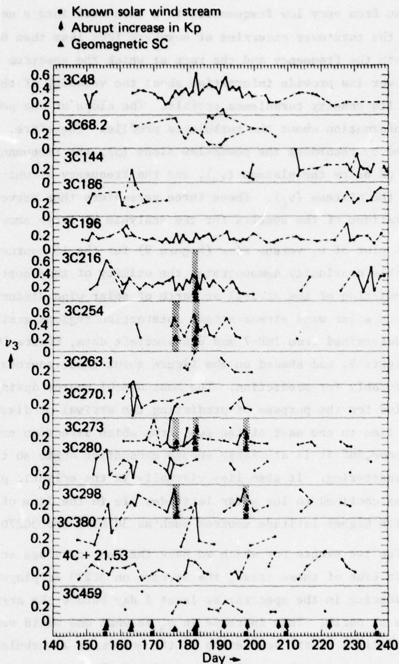
Fig. 9 \nu_3 versus time for 15 sources — known solar wind streams, SC's and abrupt increases in K_p index are indicated. The symbols are repeated (shaded) to point out the areas in the data consistent with prediction of events. On those spectra displaying two plateaus both values of \nu_3 are plotted.
