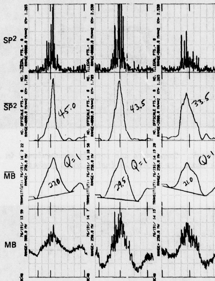
Fig. 7 Scintillation power squared (SP²) and main beam (MB) response for three successive transits of 3C48 on 1976, day 191. Unbarred variables are 2.5 second averages which are plotted chiefly to aid in the identification of interference. Barred variables are 50 second triangle weighted averages which are scaled by hand (in minor chart divisions) and then combined with the scale factor (KM) just to the left of each SP² curve to yield the scintillation index. For example, for the leftmost set of curves the scintillation index is: m = 1.789 \cdot (\sqrt{45.0})/27.0 = 0.44 . The Q values shown are quality factors which are helpful when summarizing a large number of observations.
