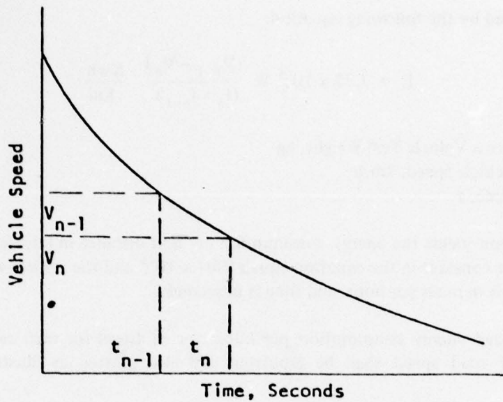
Figure A5. Vehicle speed versus time during coasting.
