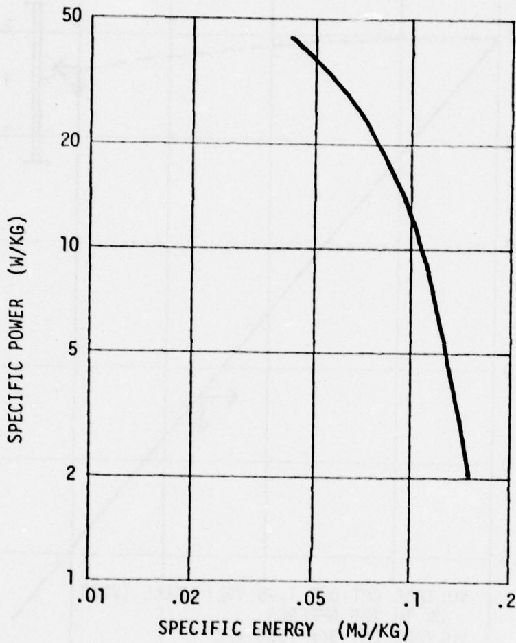
Figure 11. Battery energy/power relationship.
