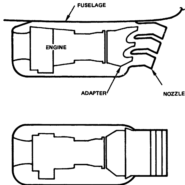
Figure 4. YAH-64/Suppressor components.
