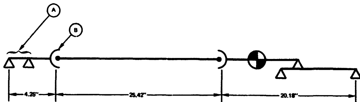
Figure 1. Schematic view of APU shaft.
