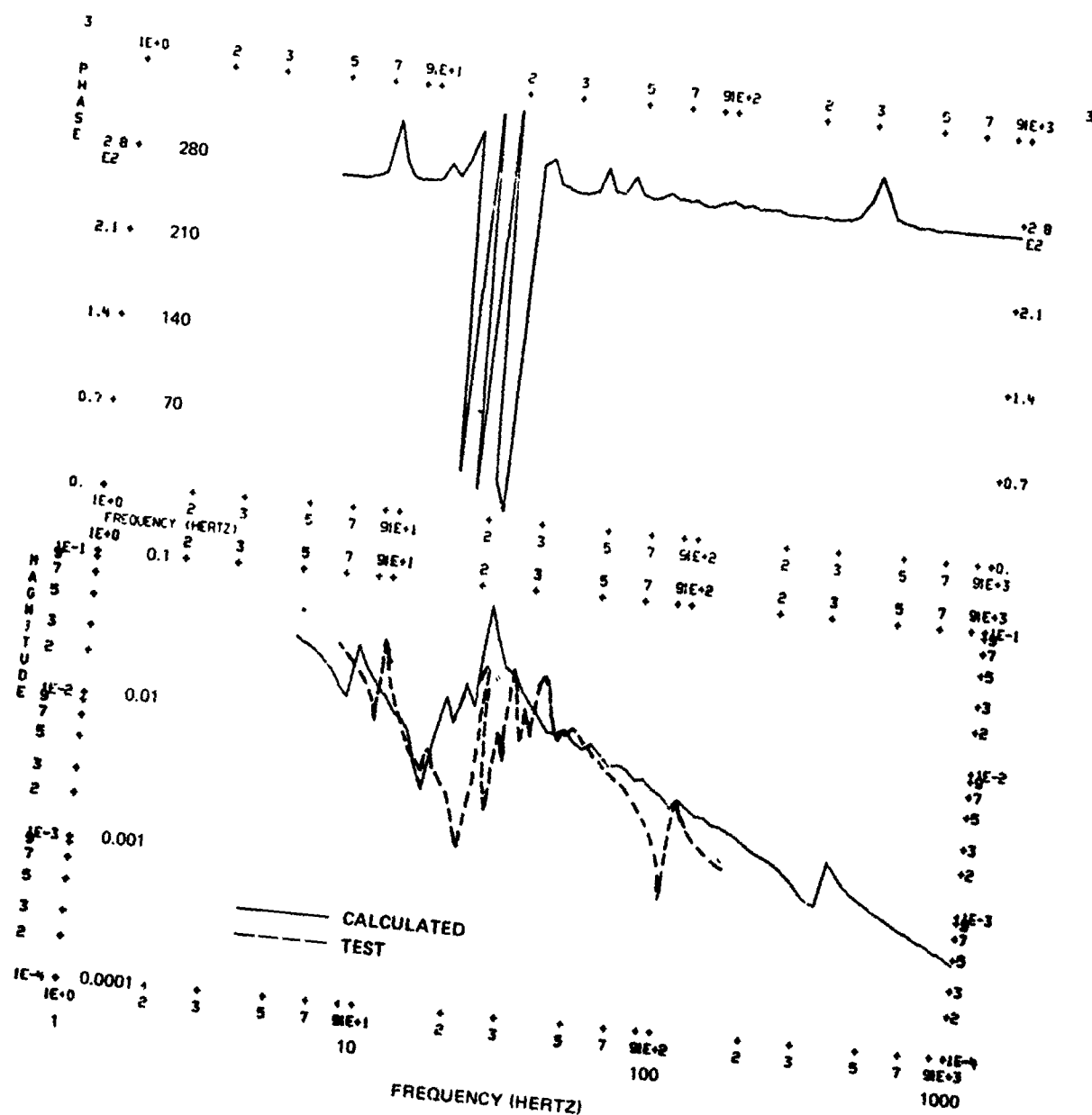
Figure 24. Direct mobility - main rotor lateral.
