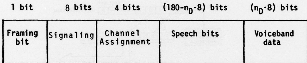
Figure 2.6 The DDR Frame.
