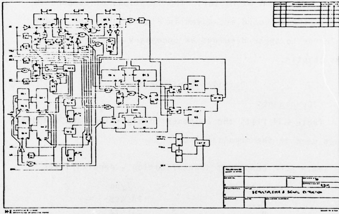
Figure 4.33 Demultiplexer schematic
