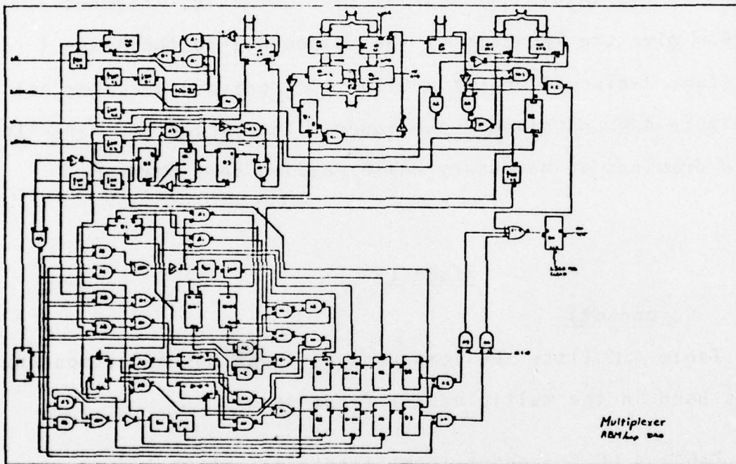
Figure 4.30 Multiplexer schematic
