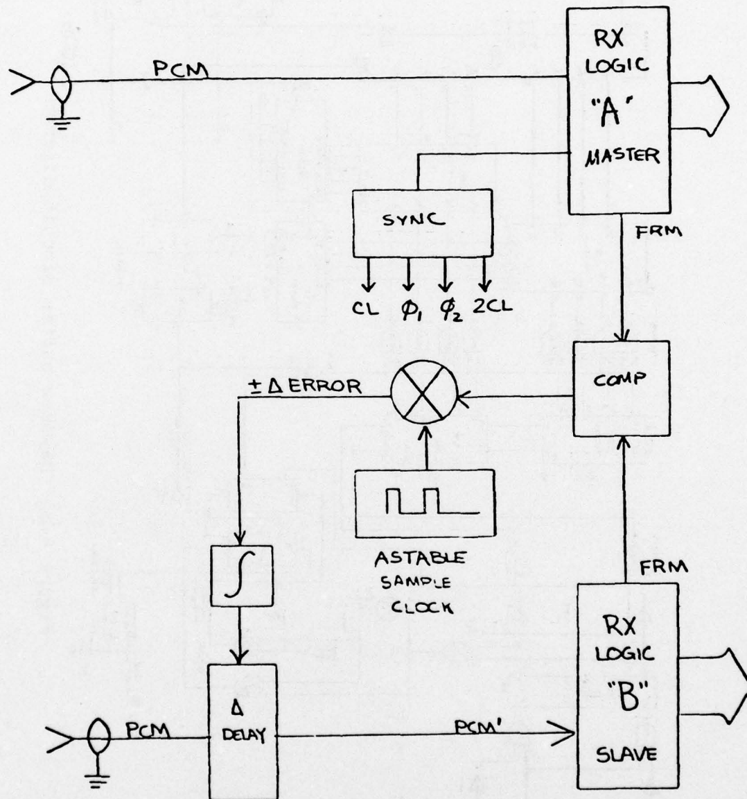
Figure 4.42 De-skew buffer
