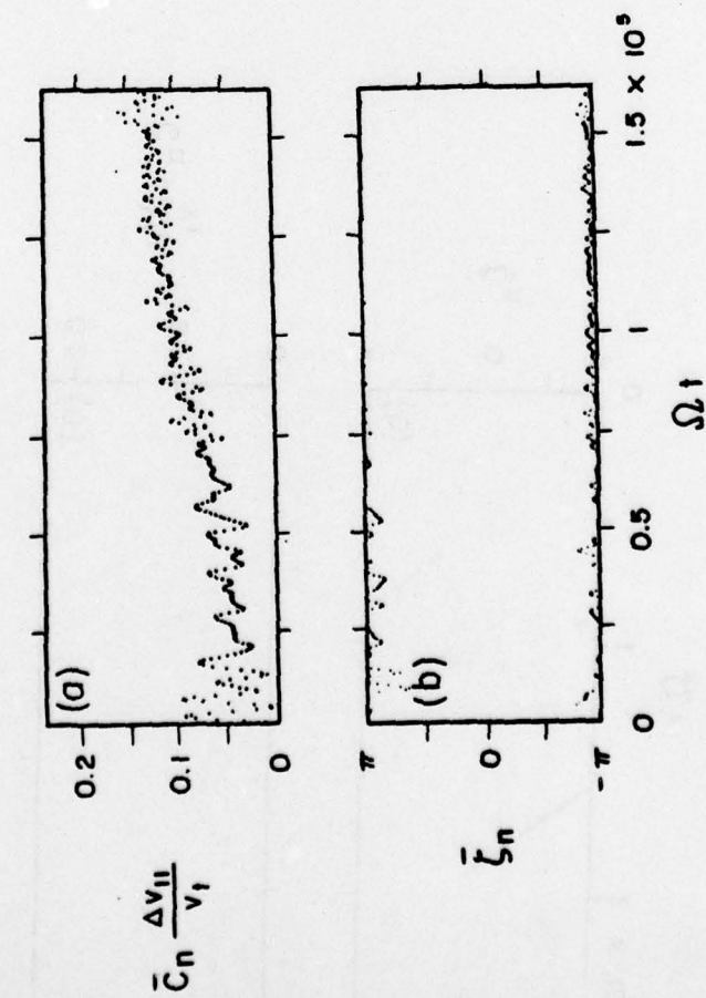
Figure 11. Amplitude, \bar{C}_n , and phase, \bar{\zeta}_n , of the correlation for the simulation of Fig. 10.
