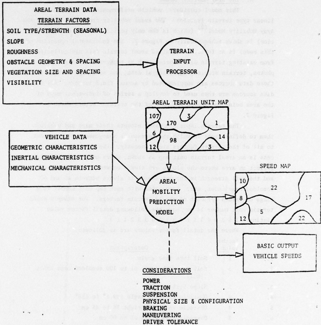
Figure 2 The Army Mobility Model (Areal Mobility Prediction)
