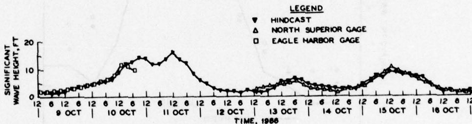
Figure 16. Comparison of time series of significant wave heights observed at Eagle Harbor for storm of 9 October 1966 and wave heights hindcast by numerical model for same storm
