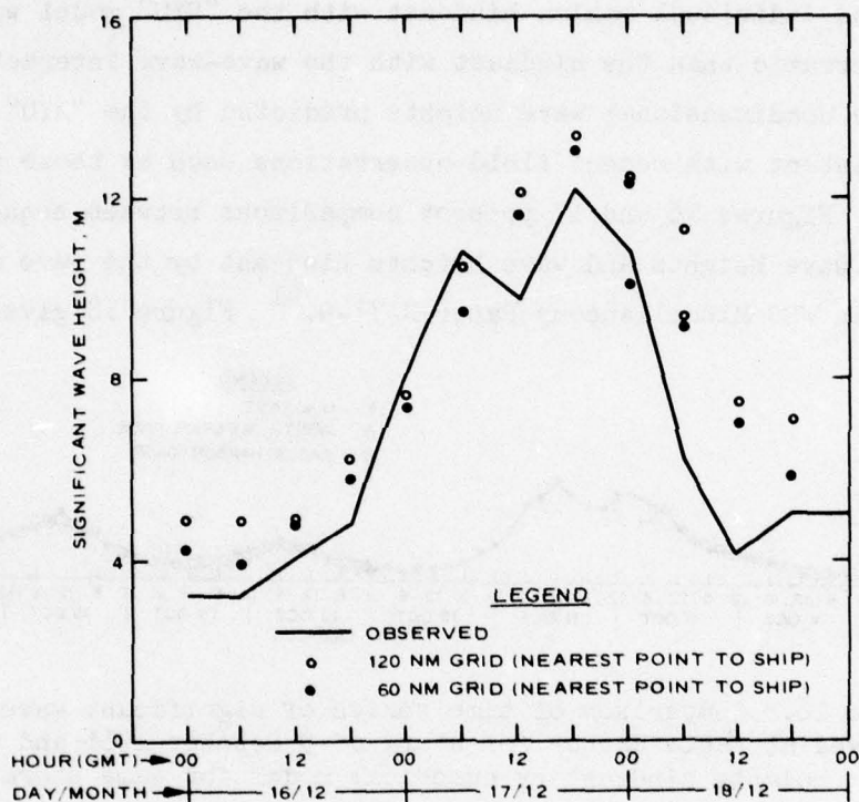
Figure 15. Hindcasted significant wave heights for 16-18 Dec 1959, using Barnett model with 60-nautical-mile grid "0" and 120-nautical-mile grid "0" as compared with observed wave heights from the OWS "Weather Reporter"
