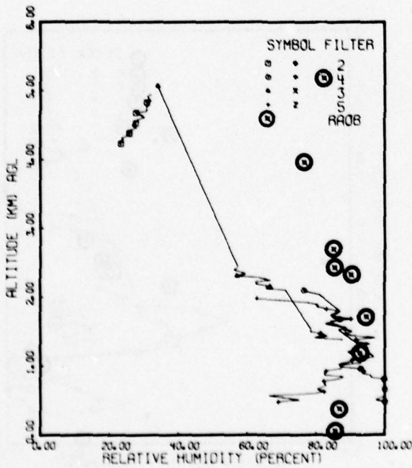
Fig. 6-3 cont. Relative Humidity Versus Altitude for Eleven Project OPAQUE II Flights.
