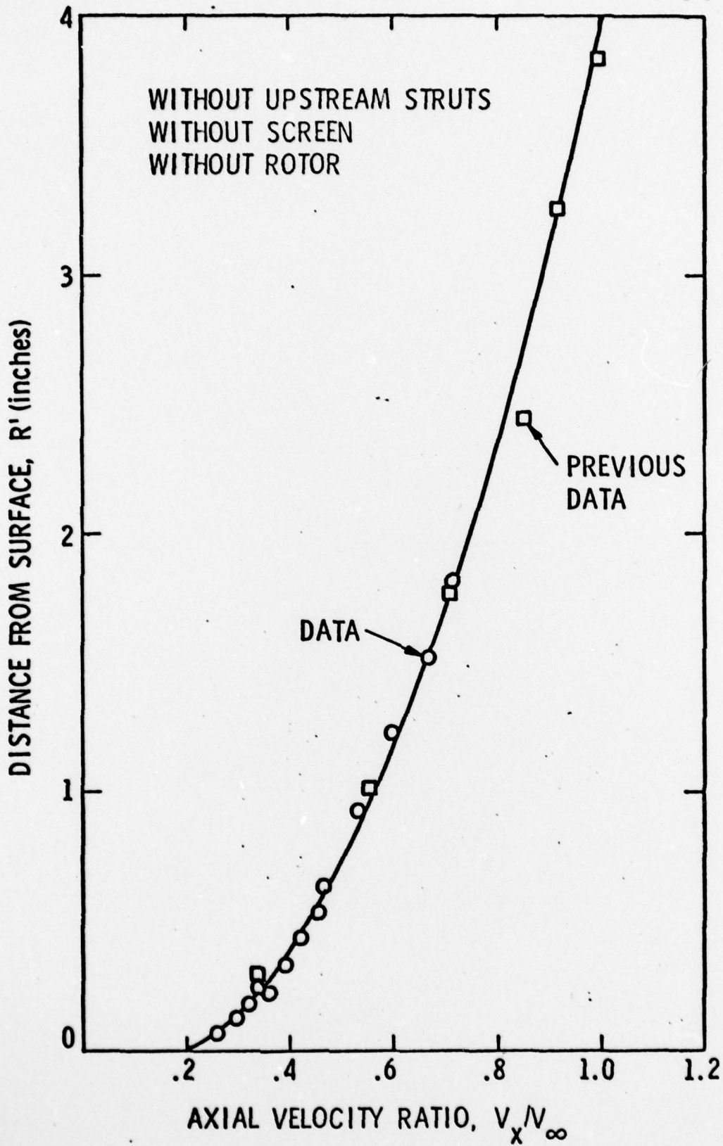
Figure 4 - Boundary Layer for Bare Body
