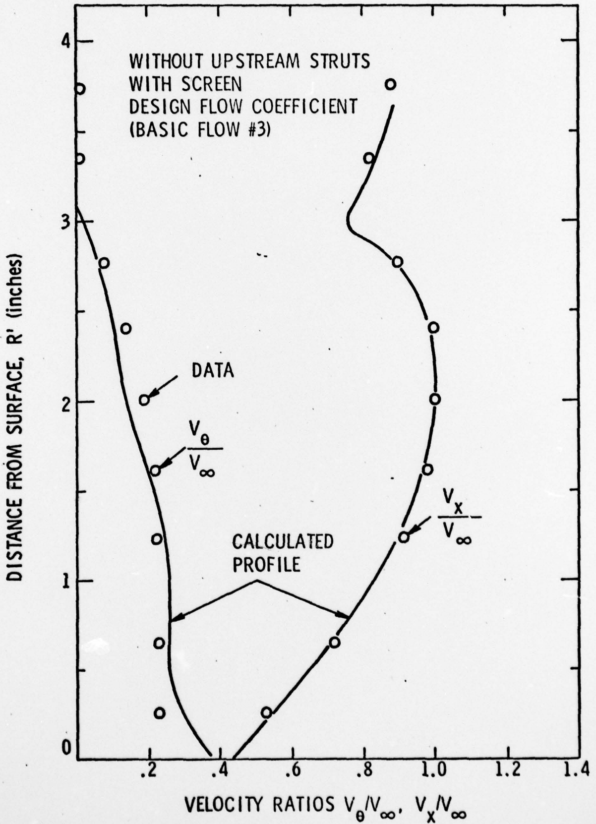
Figure 11 - Rotor Outlet Velocity Profiles for Basic Flow No. 3
