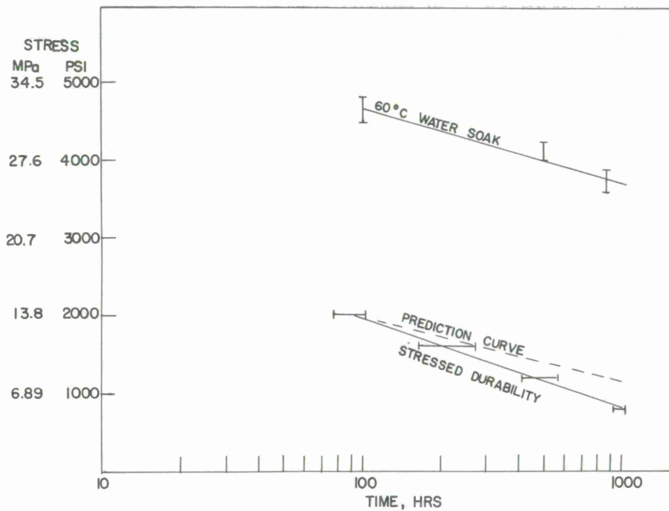
Figure 17. Comparison of 60°C water-soak residual-strength curves to stressed-durability curves for etched CP titanium alloy joints bonded with adhesive K
