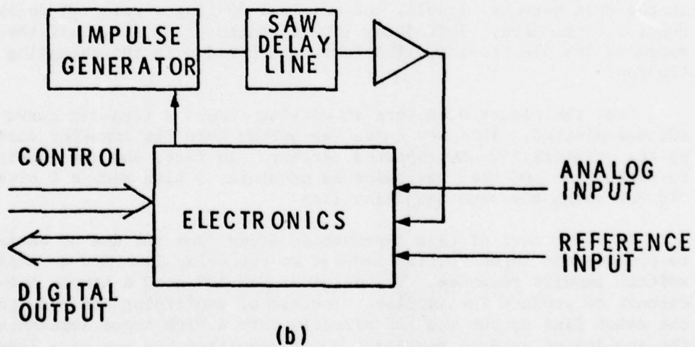
Components of SAW-ADC Subsystem
